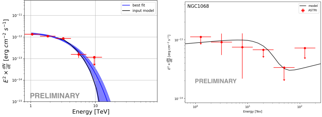
Figure 3: Left panel: spectrum of RGB J1117+202 for 200 h observations. The adopted source spectral model ( black line ) is shown superimposed to the corresponding uncertainty of the reconstructed emission profile ( blue line and shaded area ) and the observed spectrum ( red dots ). Right panel: simulated \gamma -ray spectrum of NGC 1068. The observed signal after 200 h of observation ( red dots ) is shown superimposed to the spectrum predicted by the AGN wind model ( black line ) [16, 17].
