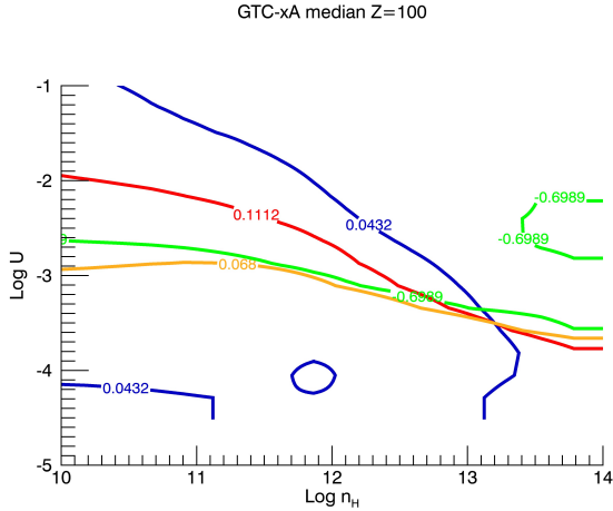
Fig. 7. Isocontours in the plane \log of ionization parameter ( U ) versus \log of hydrogen density ( n_{\text{H}} ) from CLOUDY simulations for the line intensity ratios \text{AlIII}\lambda 1860/\text{SiIII}\lambda 1892 (blue), \text{HeII}\lambda 1640/\text{CIV}\lambda 1549 (green), \text{CIV}\lambda 1549/\text{AlIII}\lambda 1860 (yellow), \text{CIV}\lambda 1549/\text{SiIII}\lambda 1892 (red) using Z = 100Z_{\odot} . Labels report the median values of the intensity ratios for the objects of the GTC-xA sample.
