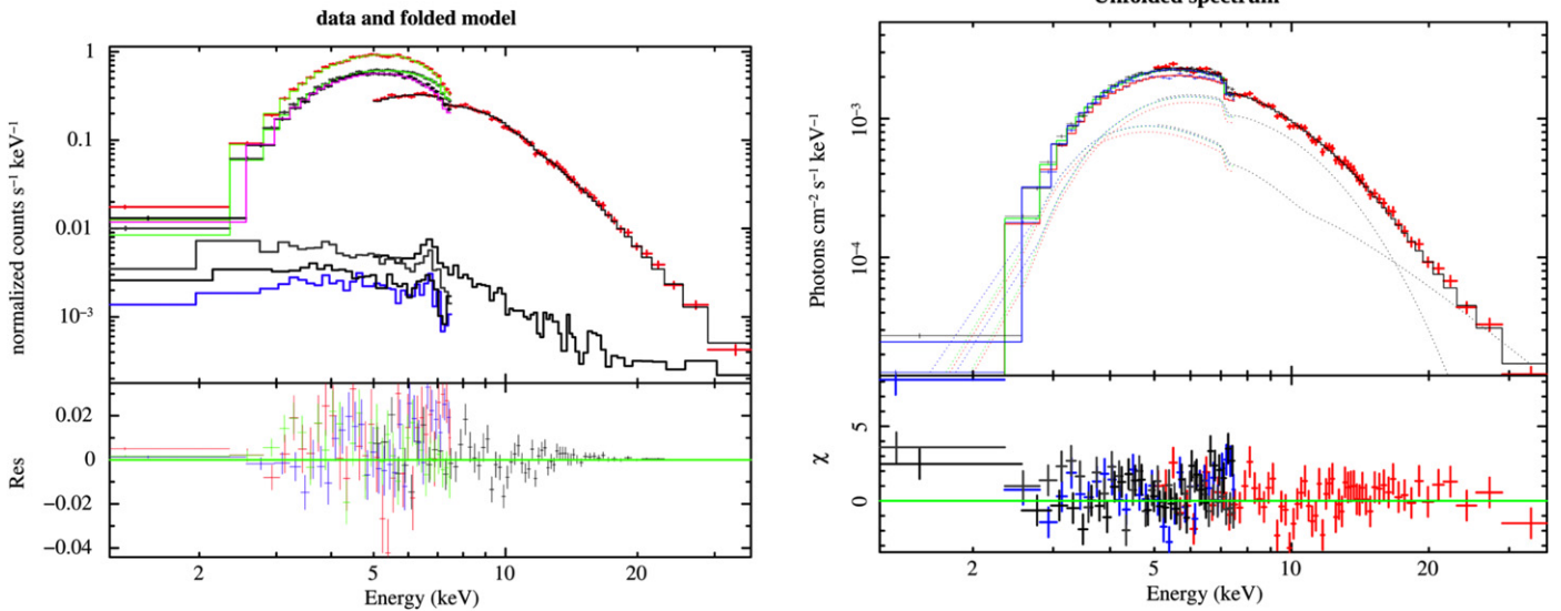
Figure 6. Left—folded spectra, backgrounds, and residuals with respect to model 4 for all of the spectra analyzed. Right—the analyzed spectra, unfolded through model 4. The plots are rebinned in groups of 30 channels for display purposes.
