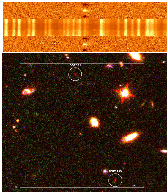
FIG. 1.— Top: the FORS2 S/N spectra of BDF521 (top) and BDF2195 (bottom) together with the reference RMS spectrum (middle). Bottom: the two objects on a HST three-color image of the BDF (blue, green and red channels are V606, I814 and Y105 respectively), the box side is of 100kpc (physical) at z=7.008 .
