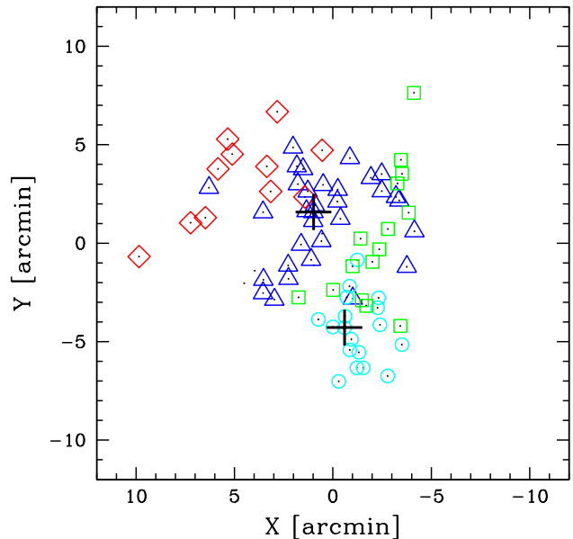
Figure 8. Spatial distribution of the 80 cluster members (small black points) within a region of \sim 2.8 \times 2.8 h_{70}^{-1} Mpc centred on the cluster center, where the galaxies of the four subclusters detected in the 3D-DEDICA analysis are indicated by large symbols. Blue triangles, cyan circles, green squares, and red rotated squares indicate galaxies of groups with increasing mean velocities. The group formed of galaxies indicated by cyan circles is the closest one to the mean cluster velocity. The members of the two main subclusters are indicated by blue triangles (the northern one) and cyan circles (the southern one). The northern subcluster stands out for its low velocity being surrounded by two high velocity groups. The two crosses indicate the two BCGs.
