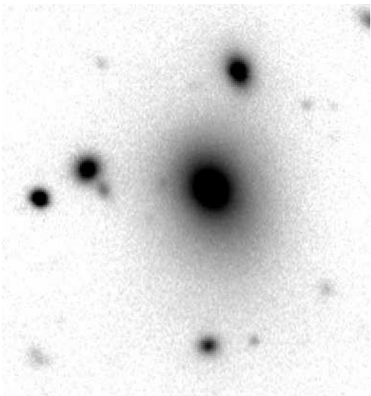
Figure 3. Zoomed-in INT r -image to view the details of the halo of BCG1, the brightest cluster galaxy specifically related to the northern subcluster. (The FOW of the image is \sim 125 \times 130 h_{70}^{-1} kpc).
