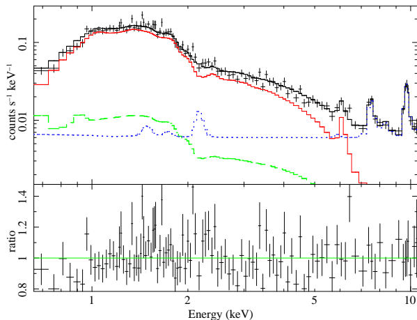
Figure 15. Upper panel: X-ray spectrum of the source taken from a 337 h_{70}^{-1} kpc aperture. The ACIS-I data are shown in black together with the best fit model with the cluster component in red (solid line), the particle background in blue (dotted line) and the sky background in green (dashed line). Lower panel: the ratio of the data over the model is also shown.
