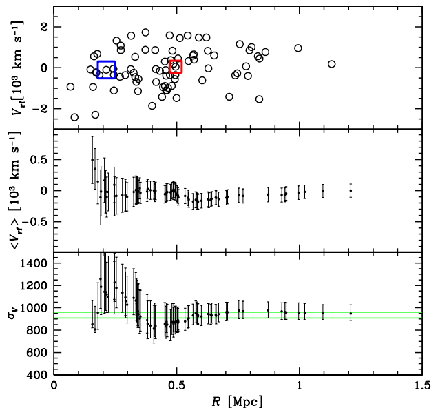
Figure 5. Top panel: rest-frame velocity versus projected cluster-centric distance for the 80 member galaxies. The very large blue square indicates BCG1 and the large red square indicates BCG2. Middle and bottom panels: integral profiles of mean rest-frame velocity and LOS velocity dispersion, respectively. The mean (and dispersion) at a given (projected) radius R from the cluster center is estimated by considering all galaxies within that radius – the first value computed on the five galaxies closest to the center. The 68% error bands are also shown. Reference values for global mean velocity and velocity dispersion are \langle V \rangle = 31\,165 \pm 107 km s ^{-1} and \sigma_v = 949_{-60}^{+80} km s ^{-1} . In the bottom panel, the horizontal, green line represents the 1sigma error band of the X-ray temperature ( kT_{\text{OUT}} = 5.3 \pm 0.3 keV, see Sect. 4.3) and converted in \sigma_v assuming energy density equipartition between ICM and galaxies, i.e. \beta_{\text{spec}} = 1 , see Sect. 6.
