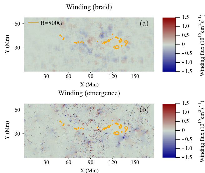
Fig. 4 Winding flux distributions of AR11318 during the plateau phase. Distributions of (a) dL_{\text{braid}}/dt and (b) dL_{\text{emergence}}/dt of AR11318 at t = 78 h. The orange contours indicate a field strength of B_z = 800 G. X and Y are distances along the x- and y-directions.
