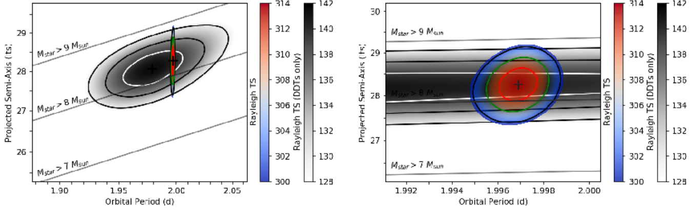
Figure 3. Contour levels of the Rayleigh test statistics in the a \sin i - P_{orb} plane. The colour (gray) scale refer to observations A+B+C (B+C) ; solid contours mark the 1, 2 and 3 \sigma confidence levels. The best estimates of the projected semi-major axis and of the period are marked with a cross. Right panel. A blow-up of the same plot around the best fit values. The solid parallel lines indicate particular configurations for which the orbital inclination and the masses of the two objects are held fixed and assuming a system observed edge-on. As the inclination of the system is unknown, these values represent lower bounds to the actual mass of the companion star.
