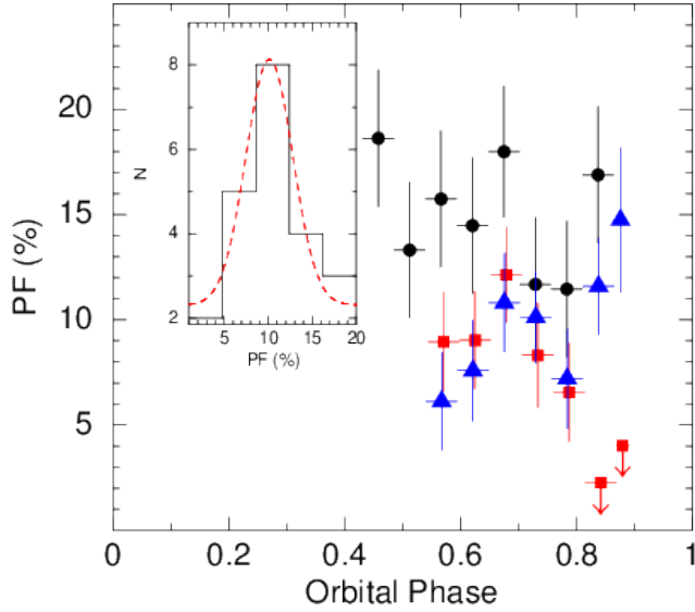
Figure 4. The evolution of the PF of M51 ULX-7 is shown as a function of the orbital phase for observations A, B and C (black filled circles, red squares and blue triangles, respectively). The histogram in the inset shows the distribution of the observed PFs, where N is the number of times the PF falls within a given percentage range (bin).
