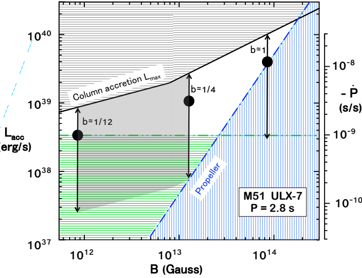
Figure 8. Accretion luminosity versus dipole magnetic field constraints for M51 ULX-7. The black solid line shows the maximum luminosity that magnetic column-accretion onto the NS can attain (Mushukov et al. 2015). The dot-dashed (blue) line marks the transition to the propeller regime, below which little (if any) accretion onto the NS surface can take place. The secular \dot{P} of M51 ULX-7, the double-dotted dashed (green) line (see the Y-axis scale on the right), is plotted here in correspondence with the minimum accretion luminosity that can give rise to it; below this line, the accretion rate would make the NS to spin-up at a lower rate than observed. Double-angled segments represent the factor of \sim 30 luminosity variations observed from the source under the assumption that they are due to accretion rate variations onto the NS surface ( L_{\text{acc}} \propto \dot{M} ); the black circle in them shows the time-averaged luminosity \langle L_X \rangle . Vertical shifts of the segments correspond to different values of the beaming factor b = L_{\text{acc}}/L_{\text{iso}} and horizontal shifts to different values of the NS dipolar surface field. For accretion to take place unimpeded down to the lowest observed luminosities level, the bottom of the segment should be above the propeller line; for the maximum observed luminosity not to exceed the maximum luminosity of magnetic column accretion the top of the segment should be below the corresponding line. Moreover only segments positions for which the circle sits above the double-dotted dashed line are allowed (otherwise the time-averaged accretion rate would not be sufficient to secularly spin-up the NS at the observed rate). The leftmost and rightmost position of the segments for which all constraints are satisfied corresponds to beaming factors of b \sim 1/12 and 1/4 , respectively (see text). Therefore the gray-shaded area between b \sim 1/12 – 1/4 and B \sim 8 \times 10^{11} – 10^{13} G represent the allowed region for M51 ULX-7 (see text). If the assumption that the luminosity follows \propto \dot{M} is relaxed, then reductions in luminosity may result at least in part from obscuration (e.g. disk precession), in which case the actual accretion luminosity range would be smaller and confined close to the top of the double-angled segments. The allowed range, besides the gray shaded area, would then extend to the white region up to b \sim 1 .
