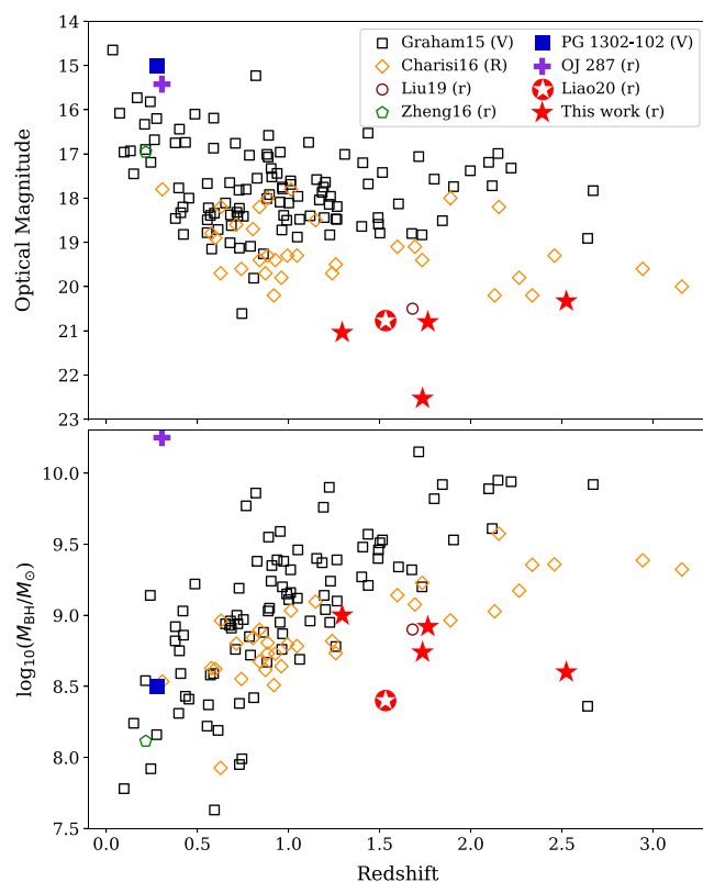
Figure 6. Top: Redshift versus optical magnitude of the four periodically variable quasars compared to those found by previous works (Graham et al. 2015a,b; Charisi et al. 2016; Zheng et al. 2016; Liu et al. 2019; Liao et al. 2020). Our candidate periodic quasars are significantly fainter than those found from previous shallower surveys in larger areas. Bottom: Redshift versus BH mass estimate. Our candidate periodic quasars are systematically less massive (with M_{\text{BH}} \sim 10^{8.4} – 10^{9.0} M_{\odot} ) than those found by previous work at similar redshifts (with M_{\text{BH}} \sim 10^9 – 10^{10} M_{\odot} ). At similar BH masses (with M_{\text{BH}} \sim 10^{8.4} – 10^{9.0} M_{\odot} ), our candidate periodic quasars are at larger redshifts ( z \sim 2 ) than those found by previous work ( z \sim 0.7 ).
