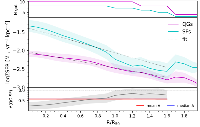
Figure 15. The SFR surface density ( \log \Sigma_{\text{SFR}} ) radial profile for QG and SF samples. The dotted black lines represent the linear fit to the radial profiles. The layout of the figure is the same as in Figure 10.
