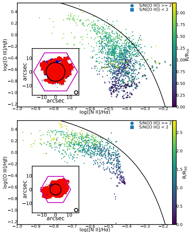
Figure 8. The resolved BPT diagram of QG 1-43012 ( top ) and of SF 1-178443 ( bottom ). Each round dot represents a spaxel in which the S/N([\text{O III}]) \geq 2 , while the square dots represent spaxels in which the S/N([\text{O III}]) < 2 and their [\text{O III}]/\text{H}\alpha values are upper-limits. The colours of the dots change according to the distance R/R_{50} of the spaxels from the centre of the galaxy. The black curve is from Kauffmann et al. (2003). The coloured maps represent the resolved BPT maps of the two galaxies. Spaxels with ionisation dominated by star formation (below the Kauffmann et al. (2003) curve) are represented in red, while those whose the ionisation is dominated by AGN/LINERs radiation are represented in blue. Overlapped is the hexagonal shape of the MaNGA IFU bundle, while the circle represents the R_{50} . The 2.5'' circle in the bottom-right corner of the maps represent the PSF (FWHM) of MaNGA datacubes.
