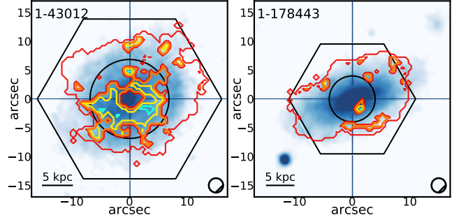
Figure 7. The contours of the resolved [\text{O III}]/\text{H}\alpha vs [\text{N II}]/[\text{O II}] diagram are superimposed to the G images (in false colours) of QG 1-43012 ( left ) and SF 1-178443 ( right ). The contours colour code is based on the position of each spaxel on the diagram, and it is the same as in Figure 1. The cyan is representing quenching regions, followed by the yellow for the galactic regions that lie between 3 \times 1\sigma and 1\sigma of the diagram, orange for those between 1\sigma and the median and red for regions of pure star-formation that are above the median of the diagram. In the bottom-left corner is reported the scale of 5 kpc. Overlapped are the hexagonal shapes of the MaNGA IFU bundles, while the circles represent the R_{50} . The 2.5'' circle in the bottom-right corner of the maps represent the PSF (FWHM) of MaNGA datacubes.
