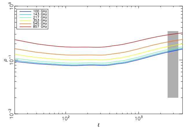
Fig. 4. Predicted correlation factor of the tSZ-CIB cross-spectrum from 100 to 857 GHz. The grey shaded area represents the range of values predicted for \rho from Zahn et al. (2012) for various models at 95, 150, and 220 GHz.
