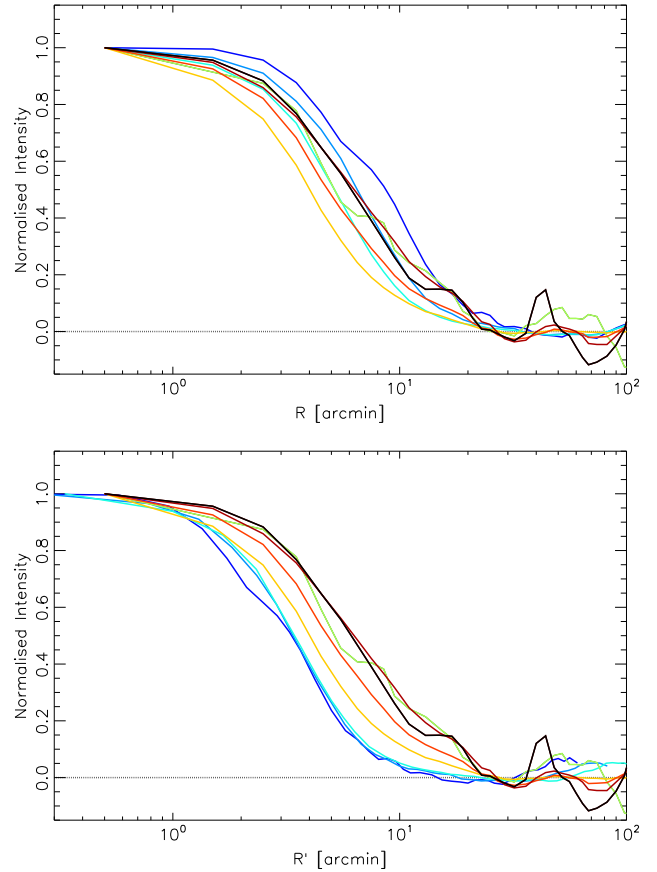
Fig. 10. Top: observed radial profile of the stacked signal toward galaxy clusters at the native angular resolution at 70 GHz (in dark blue), 100 GHz (blue), 143 GHz (light blue), 217 GHz (green), 353 GHz (orange), 545 GHz (red), 857 GHz (dark red), and 100\mu\text{m} (black). Bottom: same as top panel, but as a function of the rescaled radius R' = R(\mathcal{B}_\nu/\mathcal{B}_{857}) .
