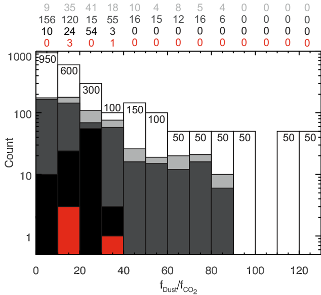
Figure 16. Histogram of the number of occurrences of activity levels NA (white), A1 (light grey), A2 (dark grey), A2 (black), and A3 (red), respectively, as a function of the dust-to-CO 2 -ice ratio. Mind that for better visibility, the ordinate is shown in logarithmic units. The numbers above the plot show, with identical colours, the number of events with activity levels A0, A1, A2, and A3, respectively. The total number of runs per bin is shown at the upper end of the white bar.
