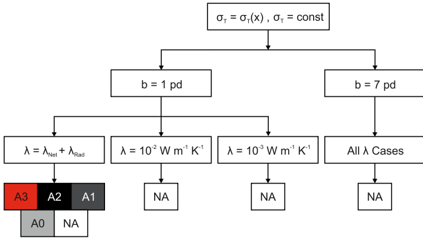
Figure 5. Overview of the different scenarios studied with our thermophysical model. In total, we studied twelve different scenarios, by varying the tensile-strength law (two cases; constant versus depth-dependent tensile strength), the gas permeability parameter (two cases; b = 1 pd versus b = 7 pd), and the thermal conductivity (three cases: \lambda = \lambda_{\text{Net}} + \lambda_{\text{Rad}} versus \lambda = 10^{-3} \text{ W m}^{-1} \text{ K}^{-1} versus \lambda = 10^{-2} \text{ W m}^{-1} \text{ K}^{-1} ), respectively. In only three of these twelve cases, dust activity (levels A0–A3; see Section 5 for details) could be measured; all other cases show no dust activity (NA).
