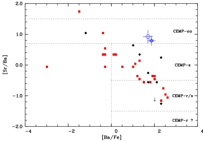
Fig. 10. [\text{Sr}/\text{Ba}] ratio of SDSS J0222–0313 (blue star for the LTE ratio and open circle for the NLTE value) compared to the CEMP sample from Hansen et al. (2016a, black diamonds) and Hansen et al. (2019, red squares), with [\text{Fe}/\text{H}] < -2.0 . Error bars for SDSS J0222–0313 are the uncertainties in [\text{Ba}/\text{Fe}] and [\text{Sr}/\text{Ba}] . We include the division (dotted lines) suggested by Hansen et al. (2019) in their Fig. 7. The star SDSS J0222–0313, being a CEMP-s star, would be expected to have a lower [\text{Sr}/\text{Ba}] value due to its high [\text{Ba}/\text{Fe}] .
