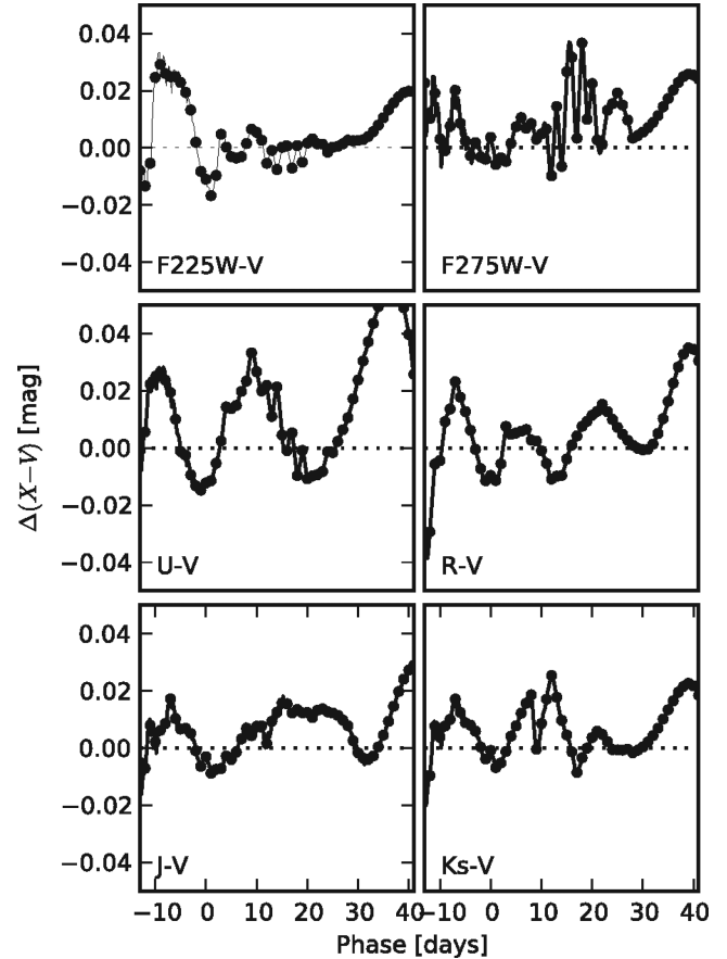
Figure B2. Examples of the difference between synthetic colours calculated from the SED template, and the corresponding colours from the light-curve spline templates.
