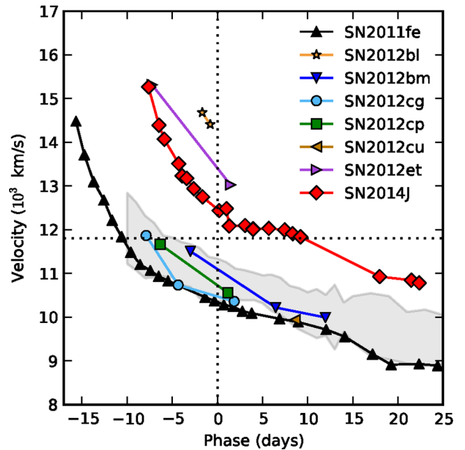
Figure 12. Measured velocities of Si II \lambda 6355 for different phases of the SNe studied in this work together with reference objects. For SN 2011fe and 2014J the velocities were calculated based on the spectra published by Pereira et al. (2013), Goobar et al. (2014) and Marion et al. (2015). The grey region is marking the average SN Ia velocity range (Folatelli et al. 2012, 2013). The dashed line marks the difference used to separate high- and low-velocity objects by Wang et al. (2009) at maximum.
