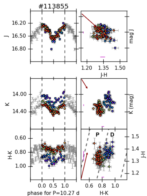
Fig. 6. Star CygOB2-113855 is an example of a disk-bearing (Class II) periodic star. With S=2.77 and ptp amplitude of 0.31 and 0.36 mag in the J and K bands, the star is also periodic in color. It is also an example of a compound variable with a variable IR-excess. The plots, colors, and symbols are the same as in Fig. 4, but with the light curves and color-curve phased with the period of the star, P=10.3 d.
