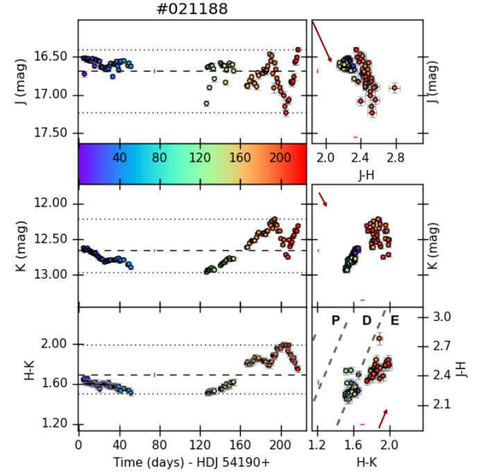
Fig. 12. Disk-bearing (Class II) star CygOB2-021188 ( S=1.0 ) is an example of compound variability showing a variable near-IR excess and a changing slope during the observed time. The plots, colors, and symbols are the same as in Fig. 4.
