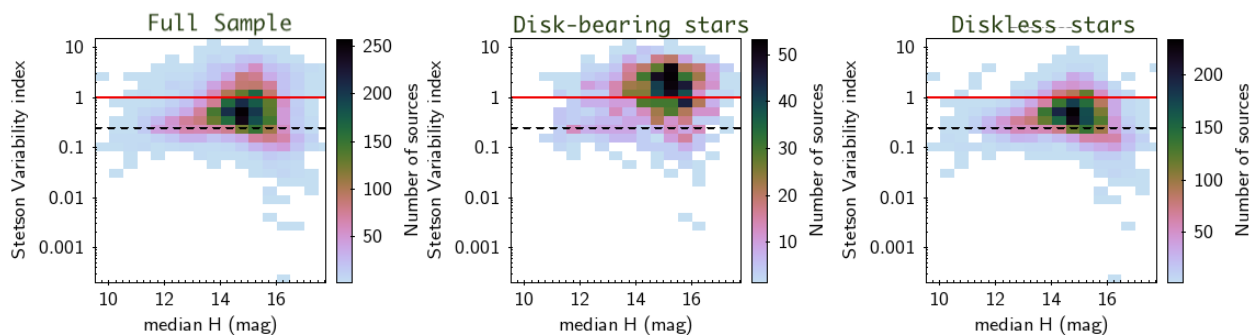
Fig. 2. Distribution of Stetson variability index as a function of H median magnitude for the full sample of candidate members (left), disk-bearing stars (middle), and diskless stars (right). The red line shows S = 1 , and the dashed black line shows S = 0.25 .
