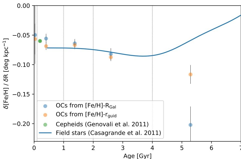
Figure 4. Age dependence of the Galactic metallicity gradient traced by open clusters in the [Fe/H]-R Gal (blue dots) and [Fe/H]-r guid (red dots) diagrams. The gradient age dependence traced by Cepheids ([31] is represented by a green circle, while field stars [119] are represented by a solid line.
