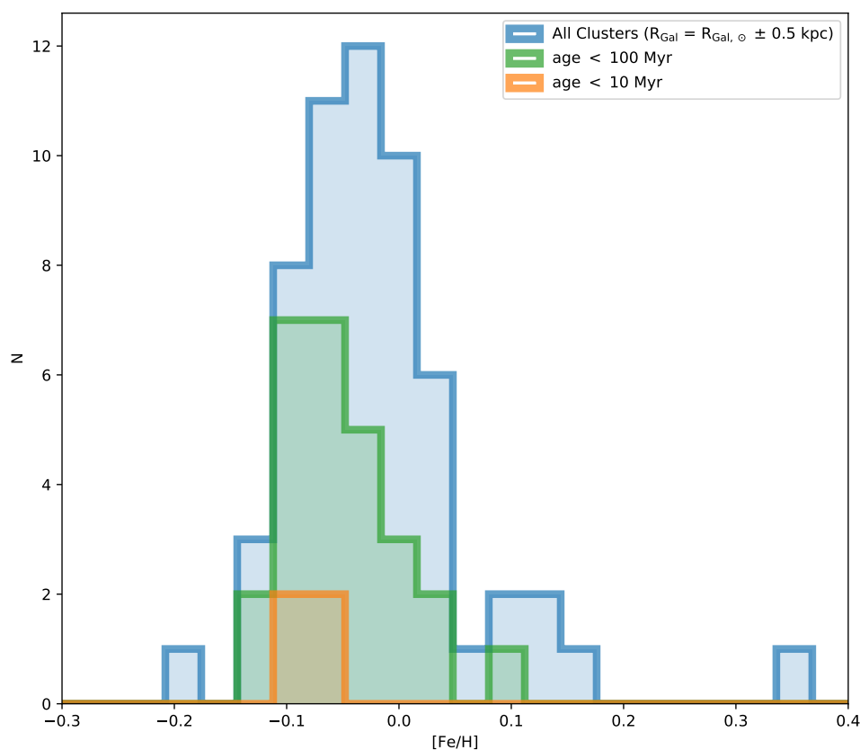
Figure 7. Metallicity distributions of open clusters from the gold sample located at R_{Gal} within R_{Gal} \pm 0.5 kpc.
