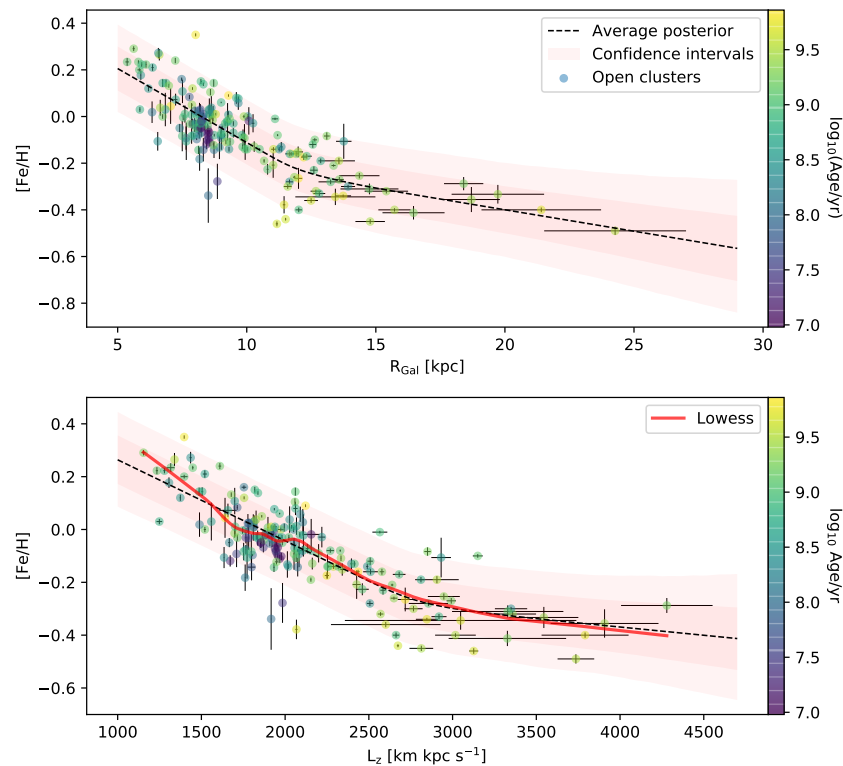
Figure 2. (Top) [Fe/H] values determined for open clusters as a function of their Galactocentric distances R_{Gal} . Clusters are colour coded as a function of their age. Red shaded areas represent the 68 and 95% confidence intervals of the models resulting from the Bayesian inference, while the black dashed line traces the most probable model. (Bottom) Same as in the top panel, but with [Fe/H] plotted as a function of angular momentum L_z .
