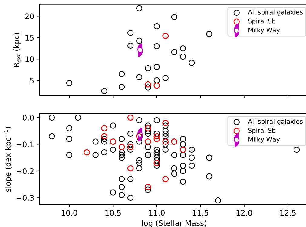
Figure 9. The figure shows the R_{ext} , the galactocentric radius at which the change of slope occurs, and the slope of the gradient in a sample of 95 spiral galaxies observed with MUSE@VLT in Sánchez-Menguiano et al. [172]. Colours and symbols are described in the legend.
