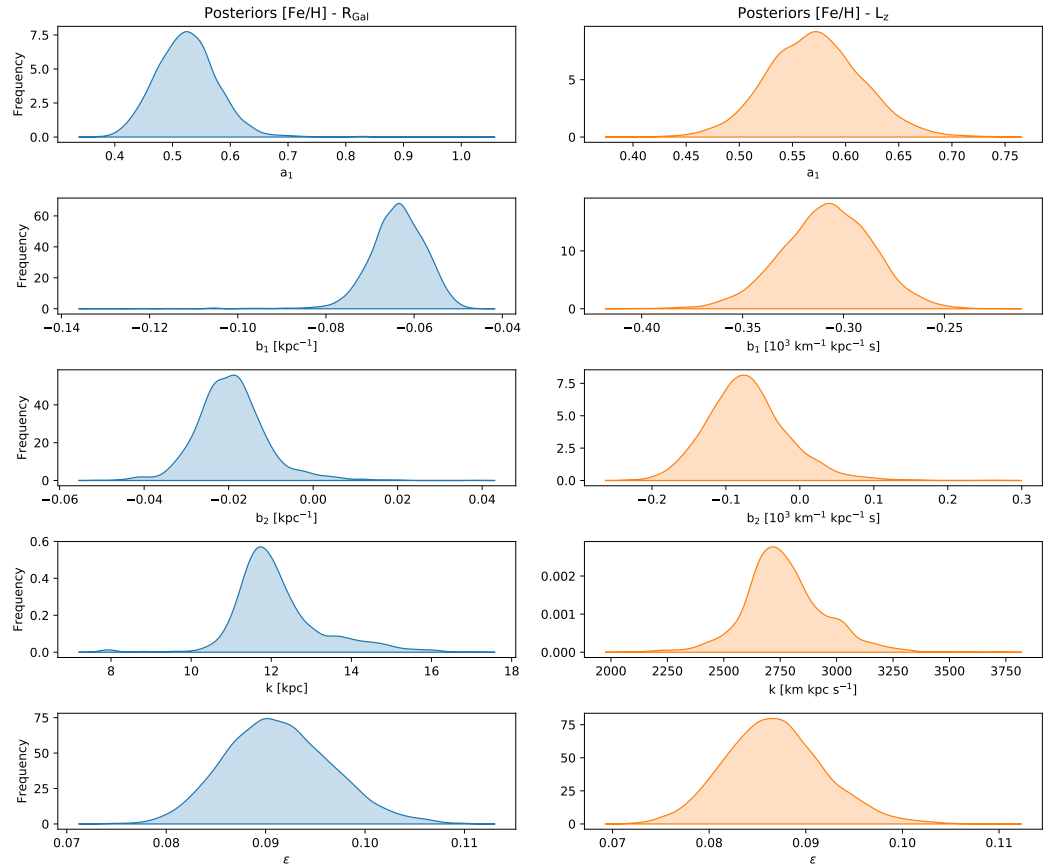
Figure 3. (Left) Posteriors resulting from the modelling in the [\text{Fe}/\text{H}]-R_{\text{Gal}} space (see Figure 2 top). (Right) Posteriors resulting from the modelling in the [\text{Fe}/\text{H}]-L_z space (see Figure 2 bottom).
