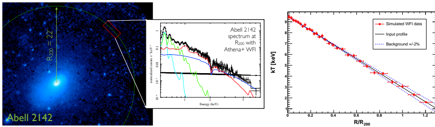
Fig. 18 capabilities of ATHENA/WFI in cluster outskirts. Left: XMM-Newton image of A2142 (Tchernin et al. 2016). The green circle shows the position of r_{200} \sim 22' . The inset shows a simulated 100ks spectrum for a 10 arcmin 2 region around r_{200} ; the red curve is the source spectrum (reproduced from Ettori et al. 2013b), reprinted with permission. Right: Simulated 100ks ATHENA/WFI temperature profile for a fiducial 8 keV galaxy cluster at z = 0.1 . The input temperature profile is shown in black and the simulated WFI data as the red data points. The upper and lower blue dotted lines show the approximate level of systematics expected in the measurements assuming a 2% reproducibility of the particle background.
