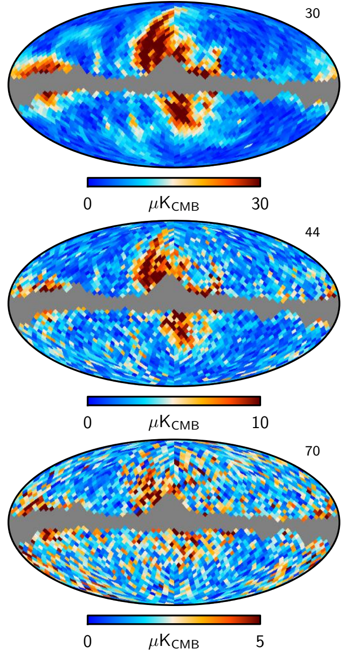
Fig. 5. Final low-resolution LFI 2017 polarization amplitude sky maps. From top to bottom , the panels show the co-added 30-, 44-, and 70 GHz frequency maps. The grey regions indicate the mask used during gain calibration. Each pixel is 3^\circ.8 \times 3^\circ.8 , corresponding to HEALPix resolution N_{\text{side}} = 16 .
