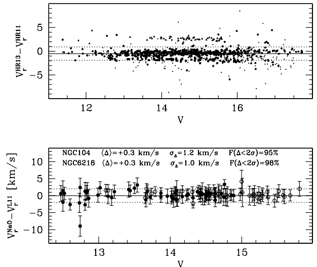
Fig. 1. Upper panel: comparison between RVs estimated from spectra obtained with the HR13 and HR11 gratings. Different symbols correspond to different clusters. The continuous line is drawn at a typical value for the mean difference ( \Delta V_r = -0.5 \text{ km s}^{-1} ), and the dotted lines enclose the \pm 2\sigma range about the mean, where a typical value of \sigma = 0.7 \text{ km s}^{-1} has been adopted (see Table 1). Lower panel: comparison with the external dataset by L11 for two representative clusters, NGC 104 (filled circles) and NGC 6218 (empty circles). The continuous line marks \Delta V_r = 0.0 \text{ km s}^{-1} , the dotted lines enclose the \pm 2\sigma range. The fraction of stars lying within \pm 2\sigma is also reported [ F(\Delta < 2\sigma) ].
