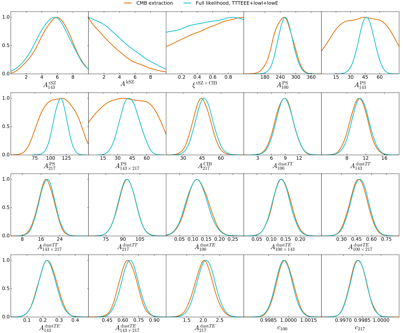
Fig. 55. Comparison of the nuisance parameters estimated simultaneously with the CMB bandpowers (red lines) and the results from the Planck likelihood (blue lines).
