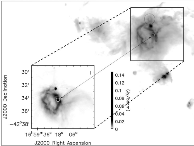
Figure 5. Composite picture of the field centred on [DBS2003] 176. The sub-panel on the bottom-left corner shows the SCORPIO map, while the background is the FIR map from Herschel (PACS, 70 \mu\text{m} ). The arrow indicates the position of the compact component SCORPIO1_300. The dotted circle in the background FIR map highlights the position of the bubble S16 (see text). In the online version a colour figure is available where the background panel is an RGB false colour image obtained from the composition of the mid-IR/FIR maps from Spitzer (IRAC, 8 \mu\text{m} , green) and Herschel (PACS, 70 \mu\text{m} , red) with the SCORPIO map (blue).
