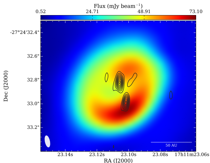
Fig. 2. Intensity contours of the 34 GHz VLA emission plotted on top of the Band 7 Stokes I image of BHB07-11. The contours correspond to intensity levels of 3, 5, 7, ... 15, 17 \times the noise level of the VLA map, 12 \mu Jy beam ^{-1} . The VLA synthesized beam of 0.10'' \times 0.04'' is shown in the lower left corner.
