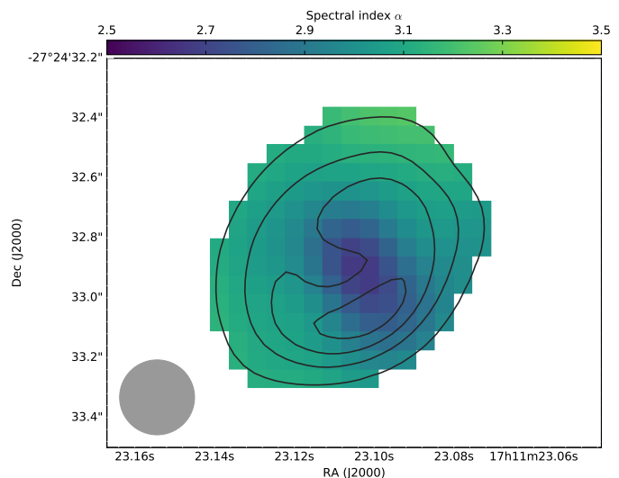
Fig. 5. Spectral index map obtained from the Stokes I emission between bands 3 and 7. The Stokes I maps were smoothed to a common circular beam of 0.25'' prior to spectral index computation. The contours show the Stokes I Band 7 flux as in Fig. 1.
