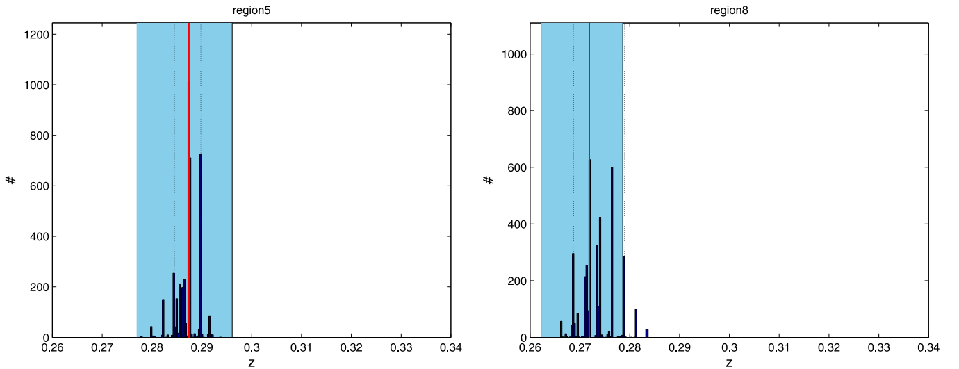
Figure 6. Histogram distribution of best-fit z_X(T_1, T_2, Z_1, Z_2) computed on the subgrid of temperature and abundance values selected as described in the text, for region 5 (left panel) and region 8 (right panel). The central vertical line shows the absolute best-fit z_X , the dashed area shows the range due to the statistical errors on the absolute best-fit z_X , and the two vertical dashed lines the lower and upper 90% percentiles of the z_X(T_1, T_2, Z_1, Z_2) distribution.
