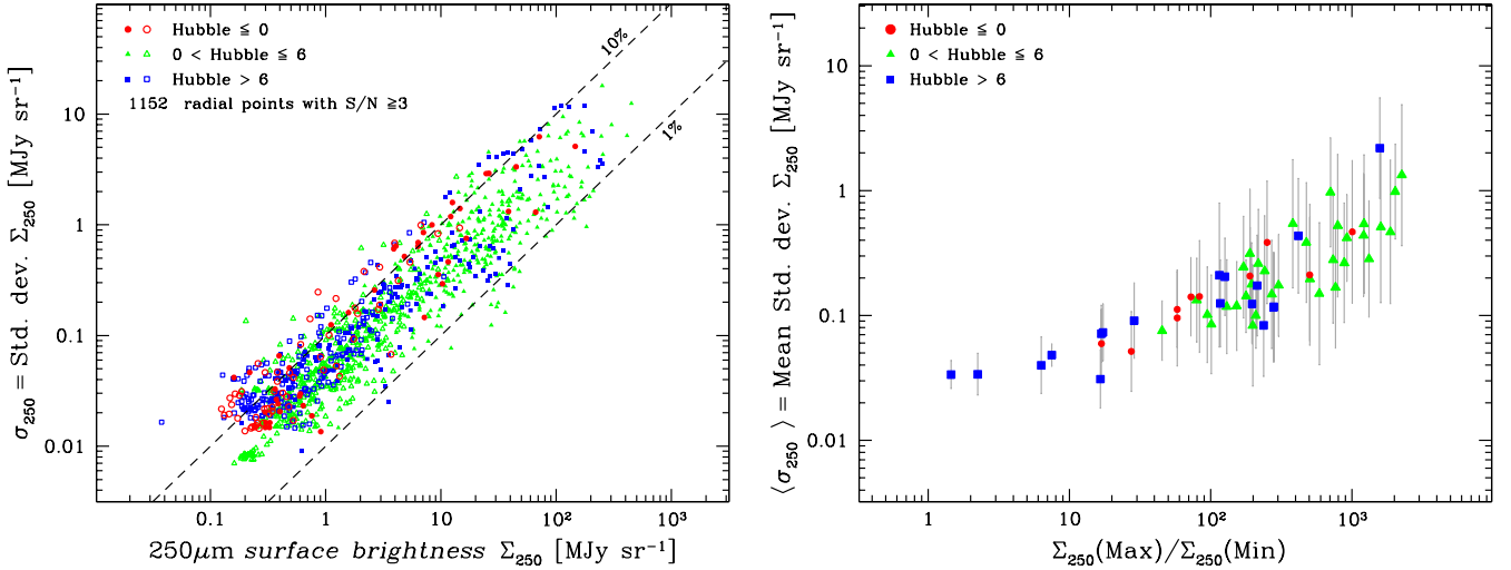
Fig. 1. Standard deviation \sigma_{250} of the 250 \mu\text{m} surface brightness within an annulus vs. 250 \mu\text{m} surface brightness \Sigma_{250} in the annulus ( left panel ), and the mean \sigma_{250} over all the profiles in a galaxy vs. the ratio of maximum and minimum \Sigma_{250} in the galaxy ( right panel ). Only radial points with S/N \geq 3 are shown. In the left panel , the dashed lines correspond to 10% variation (upper) and 1% variation (lower) relative to \Sigma_{250} . The error bars in the right panel reflect the standard deviation within a given profile. In both panels, points are plotted by Hubble type with (red) circles corresponding to early types ( T \leq 0 ), (green) triangles to spirals ( 0 < T \leq 6 ), and (blue) squares to late types ( T > 6 ); in the left panel filled symbols correspond to R/R_{\text{opt}} \leq 0.8 and open ones to larger radii.
