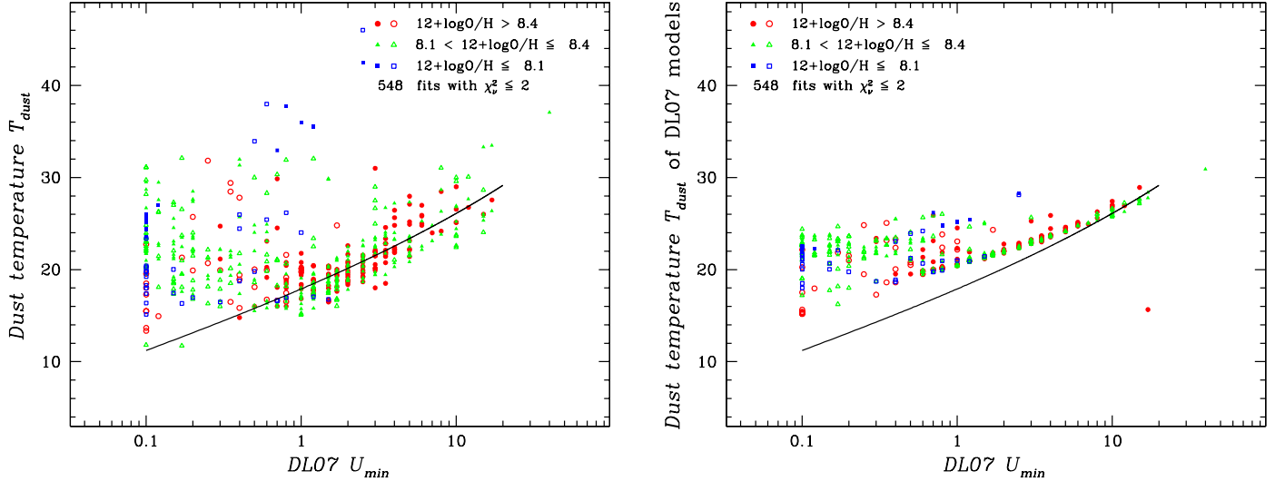
Fig. 16. Best-fit MBBV data dust temperature T_{\text{dust}} (in the left panel) and best-fit MBBV DL07 T_{\text{dust}} (in the right panel) plotted against U_{\text{min}} . Only those MBBV DL07 fits with \chi^2_{\nu} \leq 2 are considered in the plot. As before, points are coded by oxygen abundance. The curves in both panels are T_{\text{dust}} \propto U_{\text{min}}^{1/(4+\beta)} assuming the relation between \beta_{\text{DL07}} and U_{\text{min}} (see text and Fig. 15).
