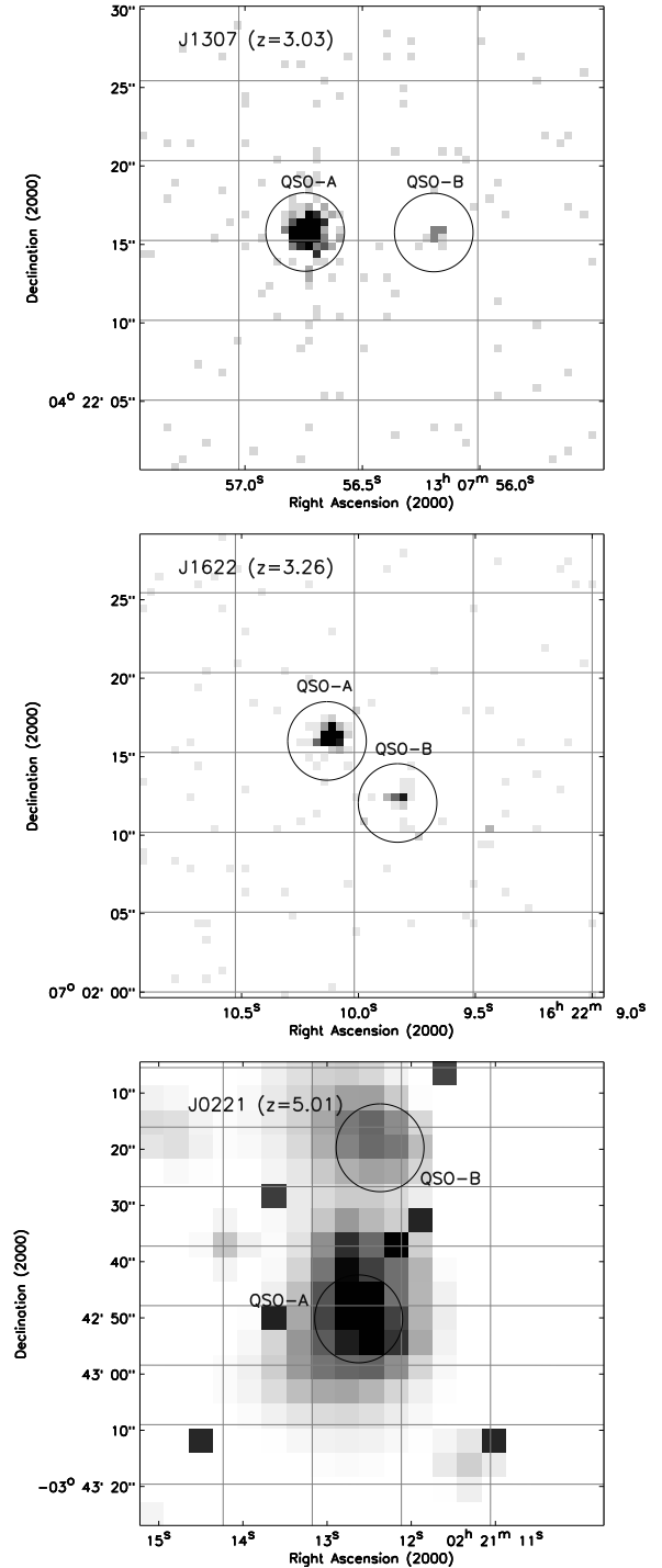
Figure 1. 0.5–7 keV band Chandra images of J1307 (top) and J1622 (middle) quasar fields. Each box side is 30'' ; the circles (diameter= 5'' ) mark the quasars of the pairs. The QSO field of J0221 as observed by XMM- Newton (pn camera, 0.3–3 keV band) is shown in the bottom panel; each side of the box is \approx 85'' , and circles have a diameter of 15'' . All images keep the original pixel size ( \approx 0.5'' for Chandra and \approx 4.1'' for XMM- Newton /pn).
