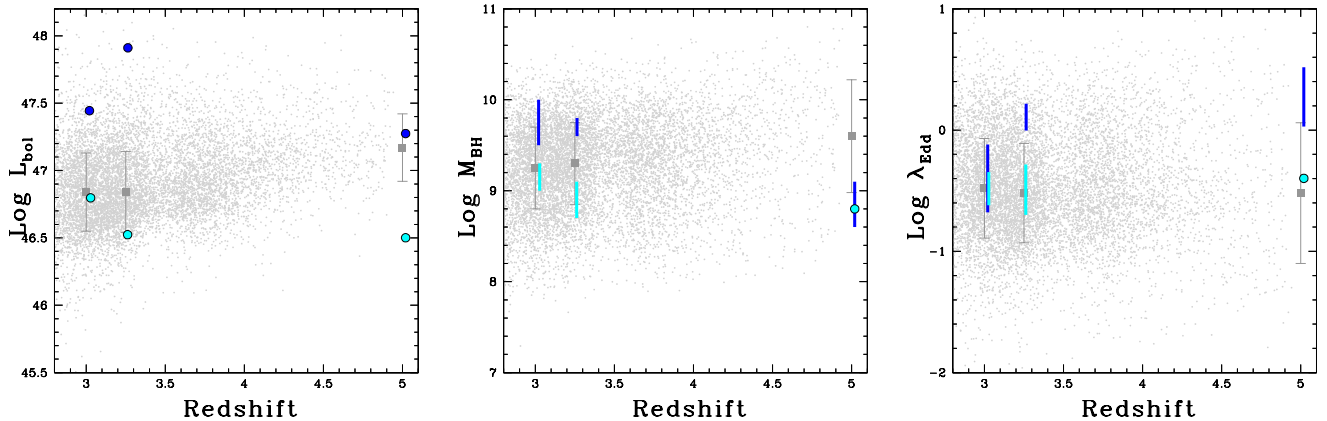
Figure 4. Comparison of the properties of the three quasar pairs of the current work vs. SDSS quasars (from the compilation of Shen et al. 2011b, updated as Nov. 2013, small grey dots): bolometric luminosity vs. redshift (left panel), black hole mass vs. redshift (middle panel) and Eddington ratio vs. redshift (right panel). The grey squares represent the median values from the SDSS quasars in redshift ranges encompassing/close to those of our sources, while the error bars show the 1\text{-}\sigma dispersion. The A (B) quasar components of our sample are shown as blue (cyan) symbols and bars; the black hole mass and Eddington ranges (excluding J0221B) are computed as described in §4, assuming negligible error on the derived bolometric luminosity (see Richards et al. 2011).
