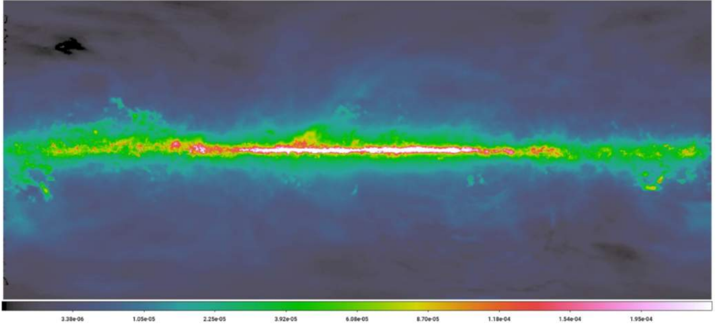
Fig. 3. AGILE diffuse \gamma -ray background emission model Giuliani et al. (2004) in the energy range 300 MeV–1 GeV, in \text{ph cm}^{-2} \text{s}^{-1} \text{sr}^{-1} , in plate carrée projection with a bin size of 0.1^\circ .
