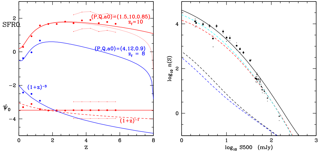
Figure 10. L: \psi_0 (lower points) and \text{SFR}_0 (upper points) as a function of redshift for quiescent galaxies (normal cirrus plus cool dust; blue) and starburst galaxies (M82 + A220 + young starburst; red) as a function of redshift, with simple analytical fits. R: differential 500 \mu\text{m} counts from HerMES and H-ATLAS surveys (Clements et al. 2010; Glenn et al. 2010; Oliver et al. 2010; Bethermin et al. 2012) compared with prediction of evolutionary model derived here. Black dashed locus: cirrus, blue: cool cirrus, red: M82 starburst, green: A220, black continuous locus: total.
