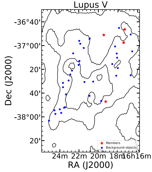
Fig. B.3. Extinction map from IRAS and COBE/DIRBE (Schlegel et al. 1998). Contours correspond to these values of E(B-V) : 0.66, 0.91, 1.17, 1.42, 1.68. The symbols of two of the members overlap.
