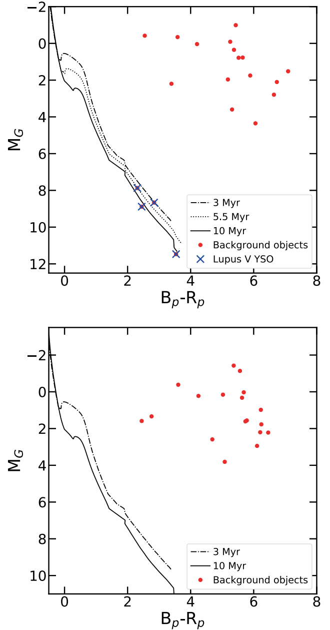
Fig. 3. Absolute magnitude vs color for the candidate YSOs in the Lupus V (top) and Lupus VI (bottom) regions with positive parallax and available Gaia magnitudes. Only the four confirmed young objects in Lupus V with available Gaia magnitudes have color and magnitudes compatible with age < 10 Myr, according to the overplotted extinction-free isochrones.
