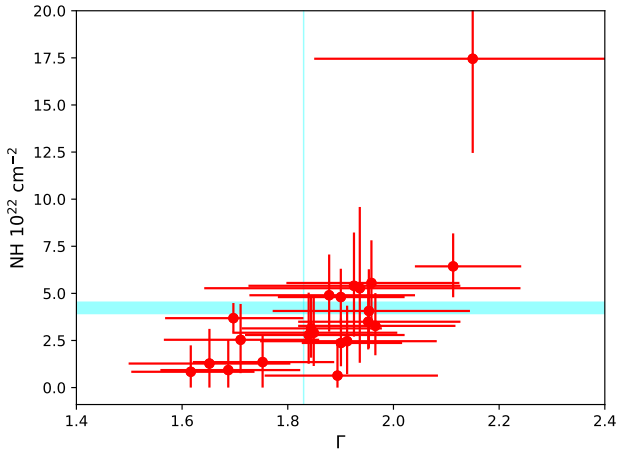
Fig. 8. Scatter plot of the best fit values of the intrinsic absorption N_{\text{H}} and the spectral slope \Gamma for each Obsid. Error bars refer to 1\sigma c.l. on a single parameter. Shaded area show the 1\sigma interval for the best fit value of N_{\text{H}} from the global fit.
