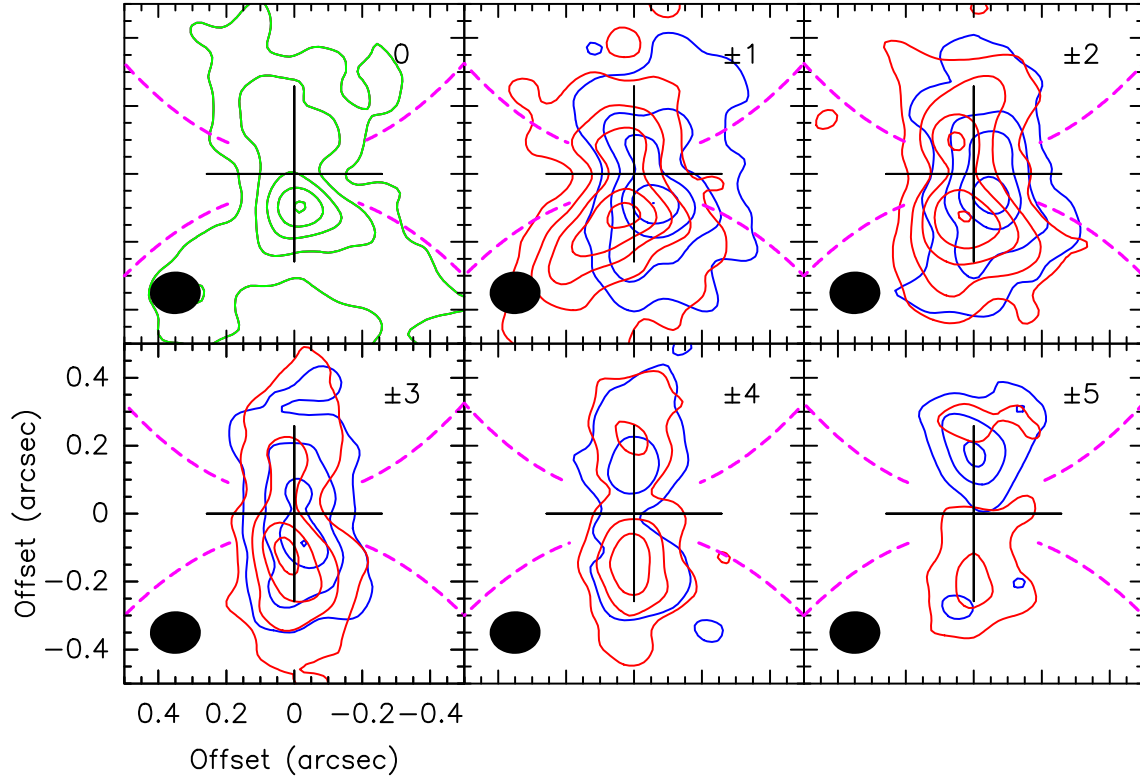
Fig. A.1. Channel maps of continuum-subtracted SO 2 8(2, 6) – 7(1, 7) emission within \pm 0.5'' of the central source of HH212. The velocity offset from the systemic velocity ( V_{\text{sys}} = 1.7 \text{ km s}^{-1} ) is indicated (in \text{km s}^{-1} ) in the upper right corner with blue and red contours denoting blueshifted and redshifted emission. The channel width is 1 \text{ km s}^{-1} . First contour and steps corresponds to 4\sigma and 6\sigma ( \sigma = 1 \text{ mJy/beam} ), respectively. The C 34 S cavity boundary from Fig. 1 is drawn in magenta dashed lines.
