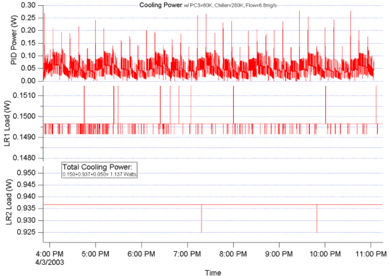
Figure 10. Cooling power data for 60K pre-cooler
