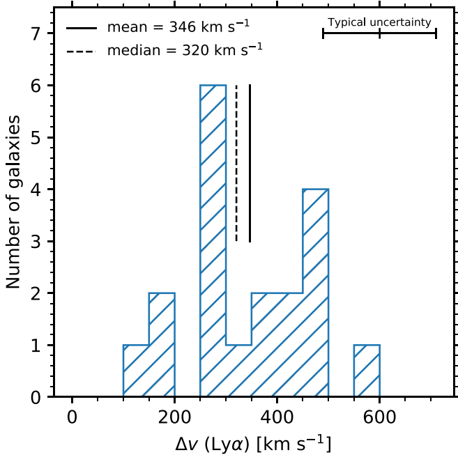
Figure 5. Histogram of the velocity offset of Ly \alpha \lambda 1216 with respect to the systemic redshift, \Delta v(\text{Ly}\alpha) . The vertical lines indicate the mean and median velocity offset in the sample. The typical \pm 1\sigma uncertainty on the velocity offset is indicated in the top right.
