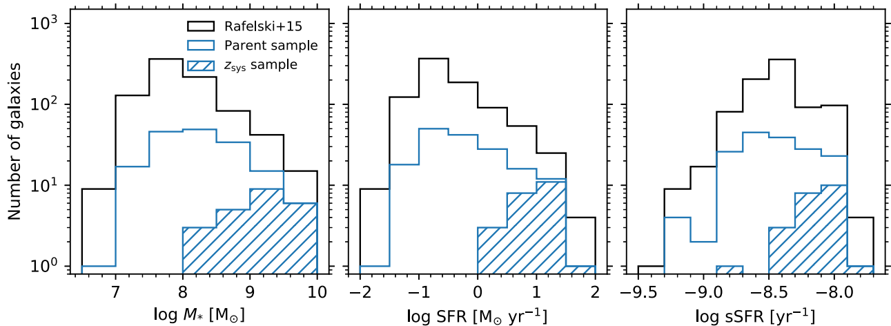
Figure 3. Histograms of the stellar mass ( M_* ), star formation rate (SFR), and specific SFR ( sSFR = SFR/M_* ) of the galaxies for which we determine a systemic redshift ( z_{\text{sys}} ), compared to the parent sample from MUSE at 3.0115 \leq z < 3.812 and all galaxies from the photometric redshift catalog by Rafelski et al. (2015).
