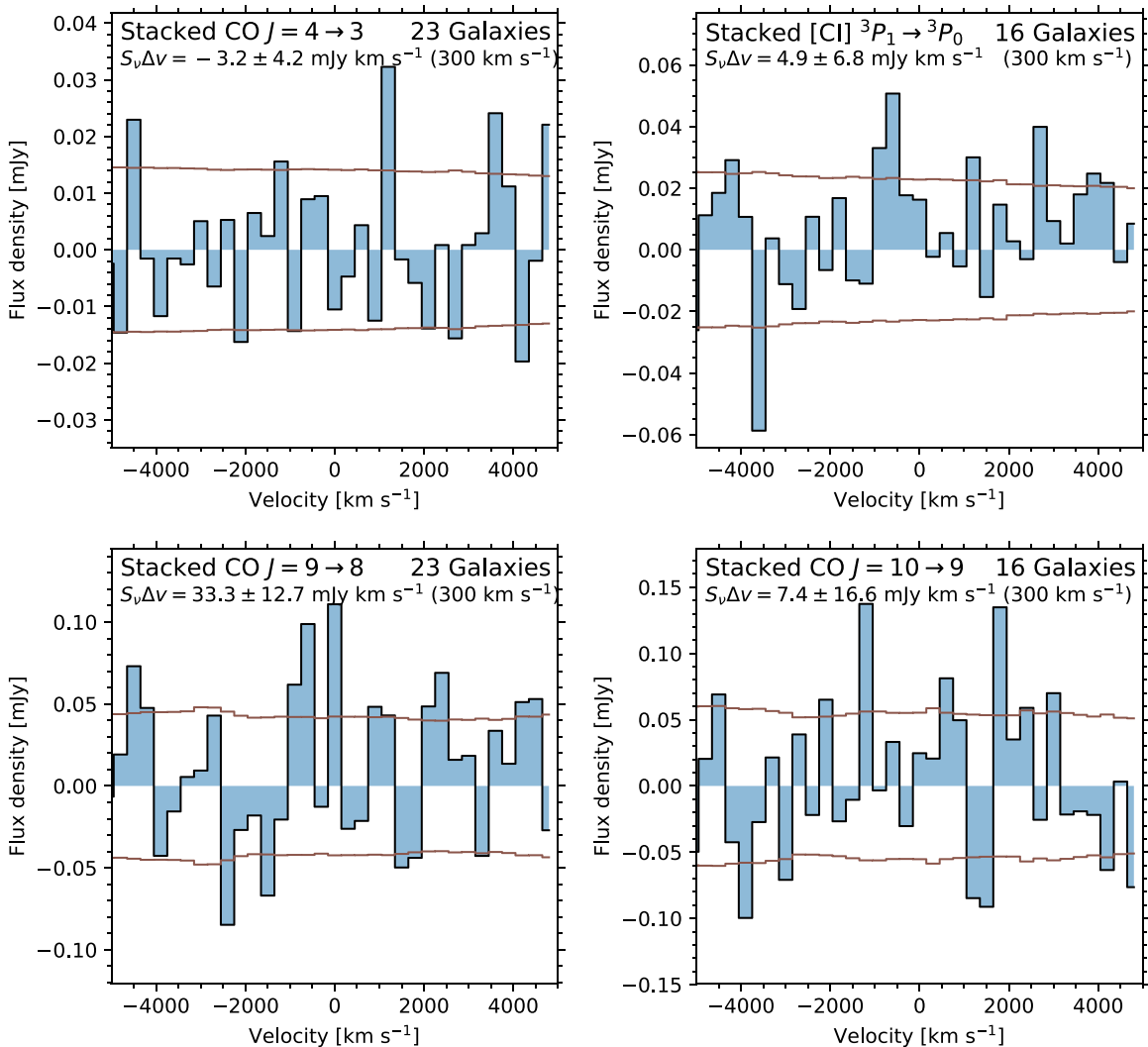
Figure 6. Stacked spectra of the ^{12}\text{CO} and [C I] transitions of the full sample. The spectrum is shown in blue and the brown line shows the rms noise (propagated through the 1/\sigma^2 weighting of the stack). The stacked transition, the number of galaxies in the stack, the integrated line flux in the zero-velocity channel, and the channel width ( 300 \text{ km s}^{-1} ) are indicated in each panel. We do not detect any emission in any of the transitions and provide 3\sigma upper limits in Table 1.
