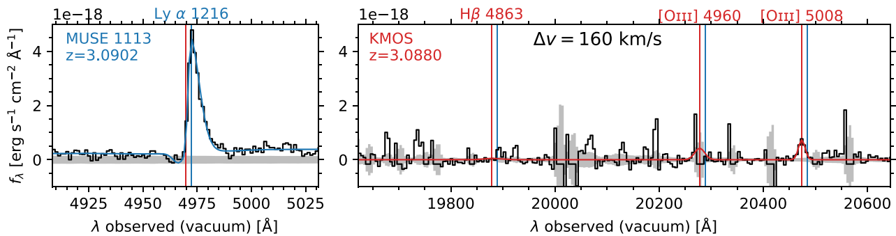
Figure 2. Rest-frame ultraviolet and optical spectra for the first galaxy in the sample with near-infrared follow-up. The left panel shows the MUSE spectrum surrounding the Ly \alpha line. The right panel shows the continuum-subtracted KMOS spectrum around the H \beta \lambda 4863 and [O III] \lambda 4960, 5008 lines. In both panels, the vertical blue and red lines indicate the redshift of Ly \alpha and the systemic redshift, respectively, determined from the fit to the spectrum (shown in the same color). This particular galaxy is detected in Ly \alpha \lambda 1216 and [O III] \lambda 5008, but not in H \beta \lambda 4863, showing a positive velocity offset between the red peak of Ly \alpha and the systemic redshift (note [O III] \lambda 4960 falls on top of a sky line). Spectra of the remaining galaxies with KMOS or MOSFIRE observations are shown in Figure 12 in Section A.
