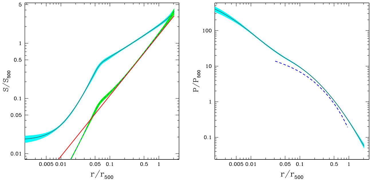
Figure 3. Left Panel: Radial entropy profile (black) and 1\sigma error region (cyan) for the fiducial hydrostatic model expressed in terms of the characteristic value S_{500} . The red line indicates the baseline r^{1.1} profile produced by gravity-only cosmological simulations (Voit et al. 2005). The black dashed line (and green 1\sigma region) represents rescaling the entropy profile by a function of the gas fraction according to Pratt et al. (2010). Right Panel: pressure profile (black) compared to the universal profile inferred for groups and clusters by Arnaud et al. (2010), which is expected to apply for the radii shown.
