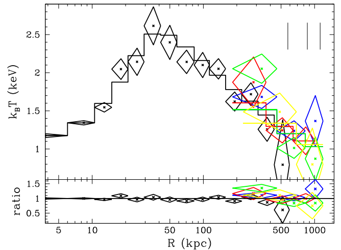
Figure 2. Projected emission-weighted hot gas temperature ( k_{\text{BT}} ) along with the best-fitting fiducial hydrostatic model in each circular annulus vs. radius R on the sky. The labeling scheme is the same as Figure 1.
