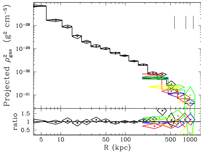
Figure 1. Quantity plotted (with 1\sigma errors) is proportional to the ICM surface brightness divided by \Lambda_\nu(T, Z) (see Equation (B10) of Gastaldello et al. 2007). The best-fitting fiducial hydrostatic model is also overplotted so that its color reflects its value for each data set. The data sets are labeled as follows: Chandra (black); Suzaku pointings: N (blue), S (red), W (green), and E (yellow). The vertical lines in the top right corner indicate the best-fitting virial radii for the fiducial model; i.e., from left to right: r_{500} , r_{200} , and r_{108} . The bottom panel plots the data/model ratio.
