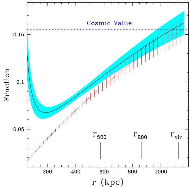
Figure 5. Radial profiles of the baryon (solid black line, cyan 1\sigma error region) and gas (dotted red line, red 1\sigma error region) fractions of the fiducial hydrostatic model.
