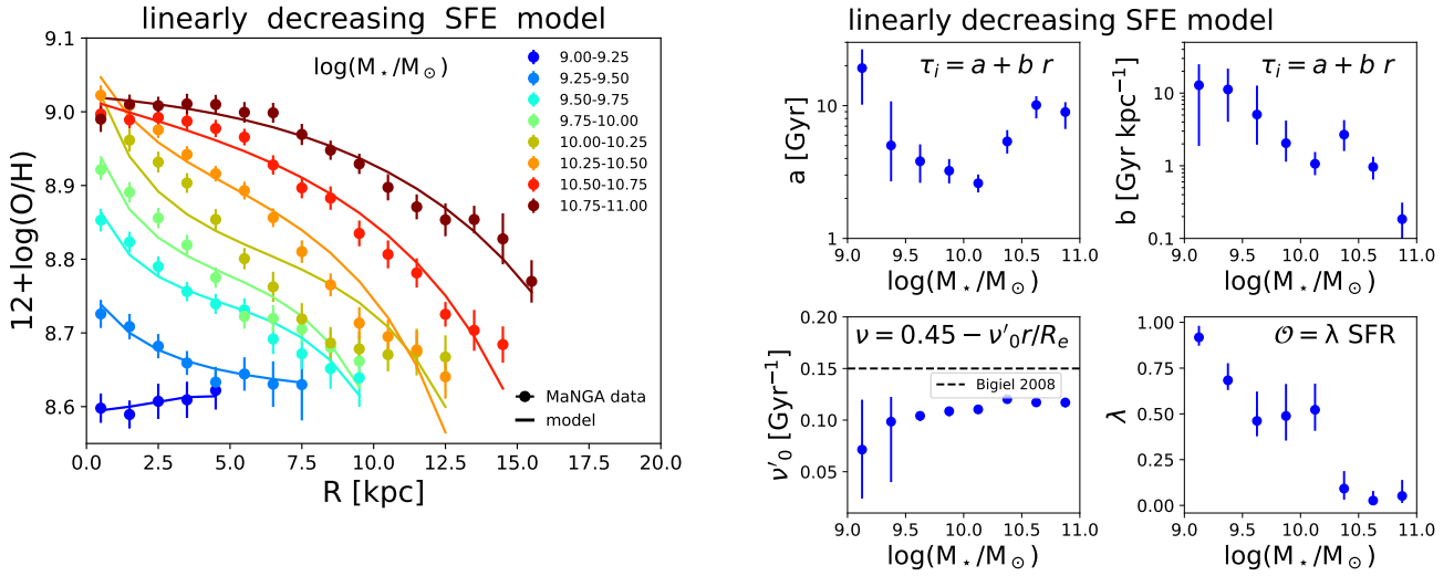
Figure 9. Left: Same as 7, but using the linearly decreasing SFE model. Right: Same as Fig. 8, but using the linearly decreasing SFE model. The parameter \nu_0 denotes the linear slope of the SFE and is compared to the median value obtained analyzing the data from Bigiel et al. (2008) for a small sample of local star forming galaxies.
