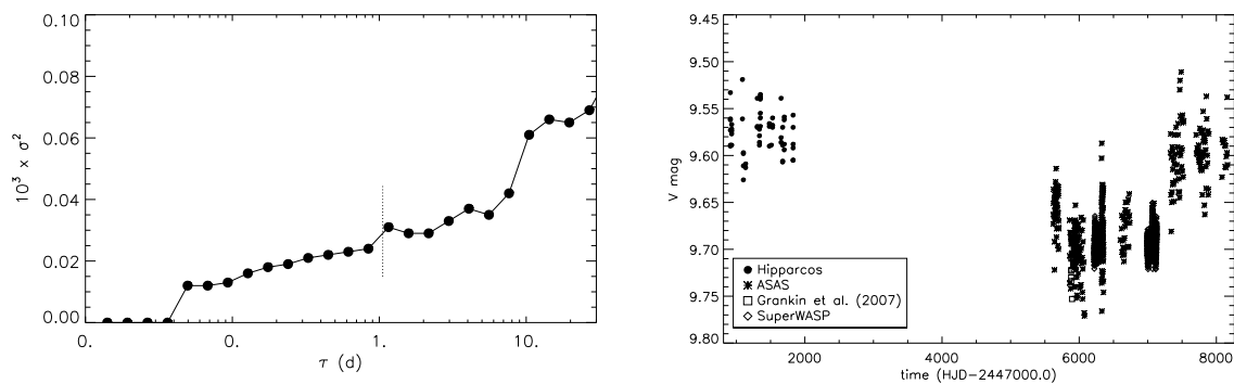
Fig. 6: Left Panel: Pooled variance profile of HD 284149 computed on the SuperWASP V-mag time series. Right Panel: Long-term V-band magnitude time series of HD 284149.
