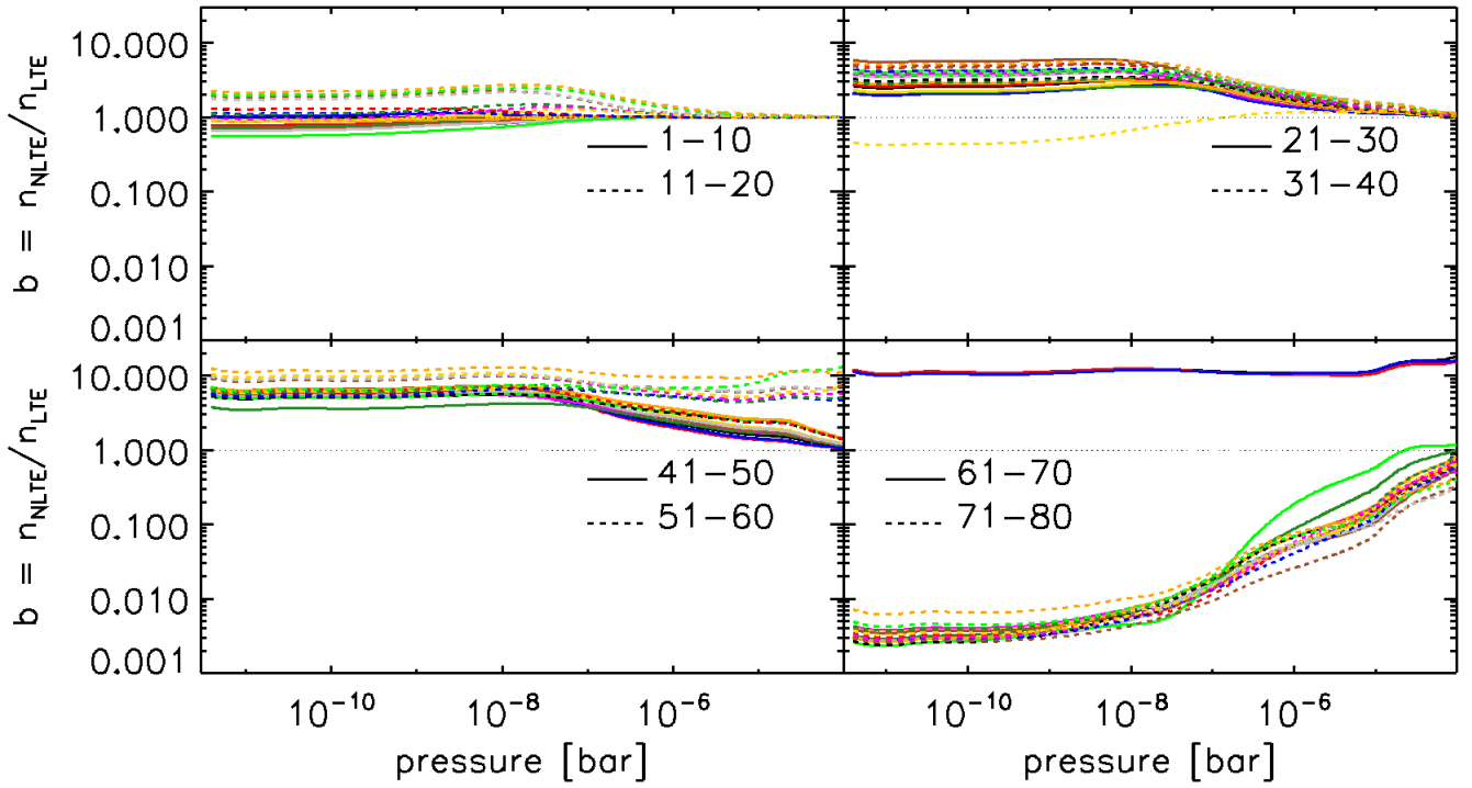
Fig. A.4. Same as Fig. A.3, but for FeII.
