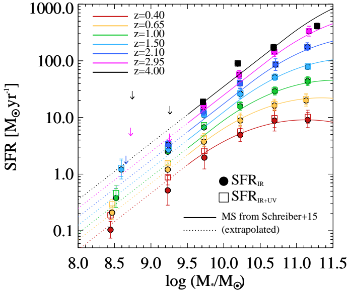
Fig. 7. SFR– M_\star relation of the NUVrJ star-forming galaxies selected in this work, colour-coded by redshift over 0.1 < z < 4.5 . At fixed M_\star and redshift, SFR IR measurements are converted from the L_{\text{IR}} obtained from IR/sub-mm SED-fitting (circles). Downward arrows indicate 3\sigma upper limits. For completeness, we also show the SFR IR+UV estimates by combining SFR IR with UV-uncorrected SFRs (open squares). Solid lines mark the evolving MS relation between SFR IR+UV and M_\star at different redshifts (Schreiber et al. 2015). We observe an excellent agreement with the MS, even below M_\star \sim 10^{9.5} M_\odot that relies upon a linear extrapolation from Schreiber et al. (2015) that is not constrained by previous data.
