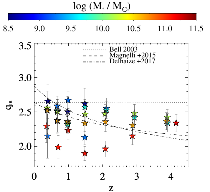
Fig. 8. AGN-uncorrected q_{\text{IR}} evolution as a function of redshift (x-axis) and M_{\star} (colour bar). Errors on q_{\text{IR}} represent the 1\sigma scatter around the median value, estimated via bootstrapping over L_{\text{IR}} and L_{1.4\text{GHz}} . For comparison, other IRRC trends with redshift are taken from the literature (black lines): Bell (2003, dotted); Magnelli et al. (2015, dashed); Delhaize et al. (2017, dot-dashed). Our q_{\text{IR}} values still include the contribution of radio AGN. See Sect. 4.1 for details.
