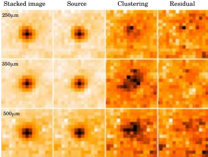
Fig. 5. Image decomposition of median stacks at 250, 350, and 500 \mu\text{m} , for a specific bin at 0.8 < z < 1.2 and 11 < \log(M_*/M_\odot) < 12 . From left to right: the stacked image is separated among a point source PSF, the clustering signal, and a residual background term, respectively. The colour scale is normalised to the maximum in each cutout for visual purposes. See Sect. 3.2 for details.
