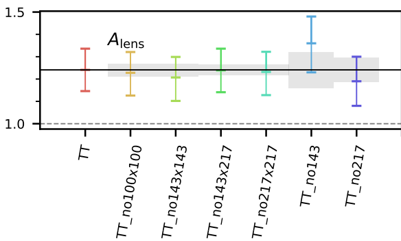
Fig. 83: Marginal means and 68 % error bars for the A_L consistency parameter for PlikTT combined with Commander and SimAll EE, when removing either a single cross-spectrum, or all cross-spectra within a given frequency channel from the high- \ell part of the likelihood (i.e., Plik). Grey bars represent the variance with respect to the full-frequency case, computed using Eq. (61).
