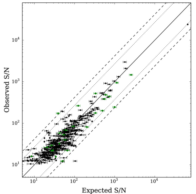
Figure 7. A comparison of the observed S/Ns of known pulsar re-detections with their predicted values. The solid line shows the expected 1:1 correlation. The dotted and the dashed lines mark the region containing 95 and 99 per cent of the data points. Pulsars with \text{DM} \leq 100 \text{ cm}^{-3} \text{ pc} are potentially affected by scintillation and are coloured in green. The error bars reflect the published uncertainties in the pulsar flux densities from PSRCAT.
