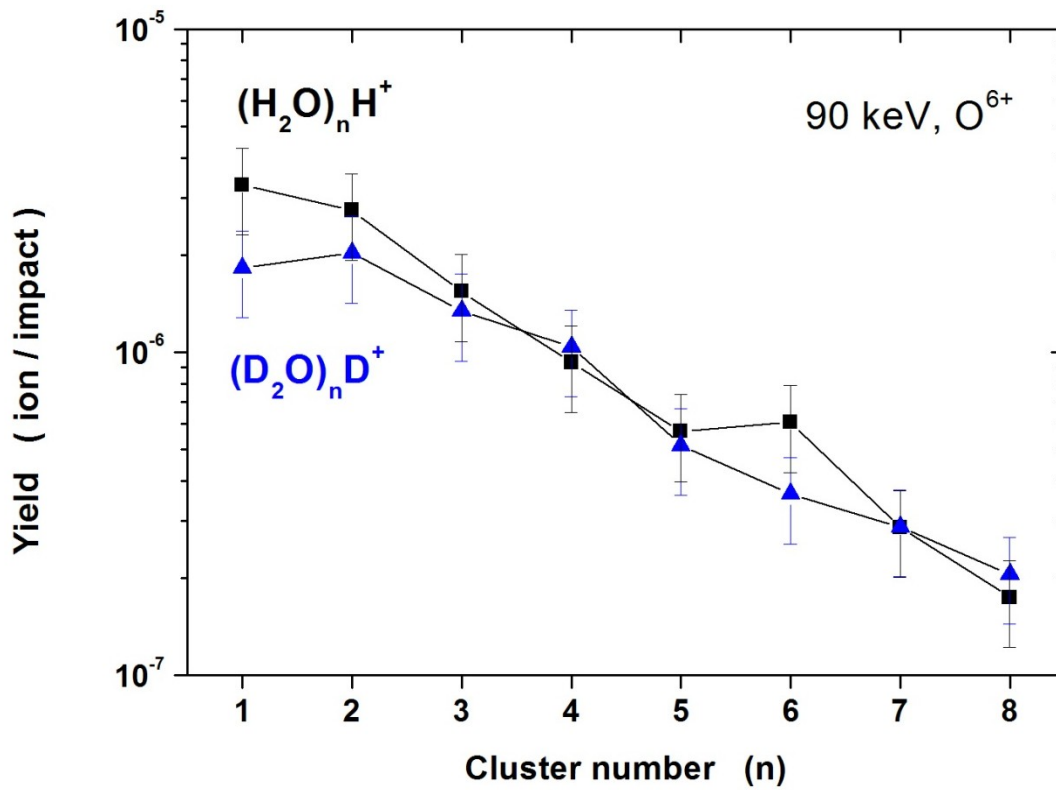
Figure 6. Secondary Total Ion Yields of (\text{H}_2\text{O})_n\text{H}^+ and (\text{D}_2\text{O})_n\text{D}^+ clusters (with n=1-8) emitted from water and deuterated water respectively. Both samples have been deposited and irradiated at 10 K.
