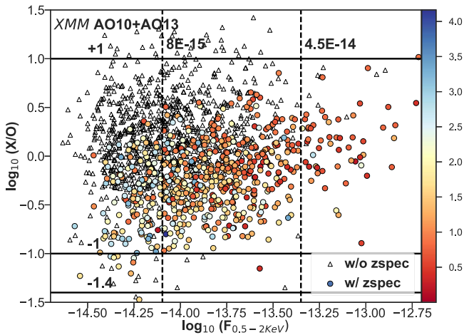
Figure 9. Log of the X-ray-to-optical flux ratio vs. the log of the soft X-ray flux (0.5–2 keV band) of all point-like objects in XMM AO10 and AO13. The ratio X/O is based on the soft X-ray flux and the SDSS i -band flux. The spectroscopic sample is color-coded by redshift. This plot shows that the spectroscopic sample tends to be brighter than the nonspectroscopic sample, although they span the same range in flux and redshift.
