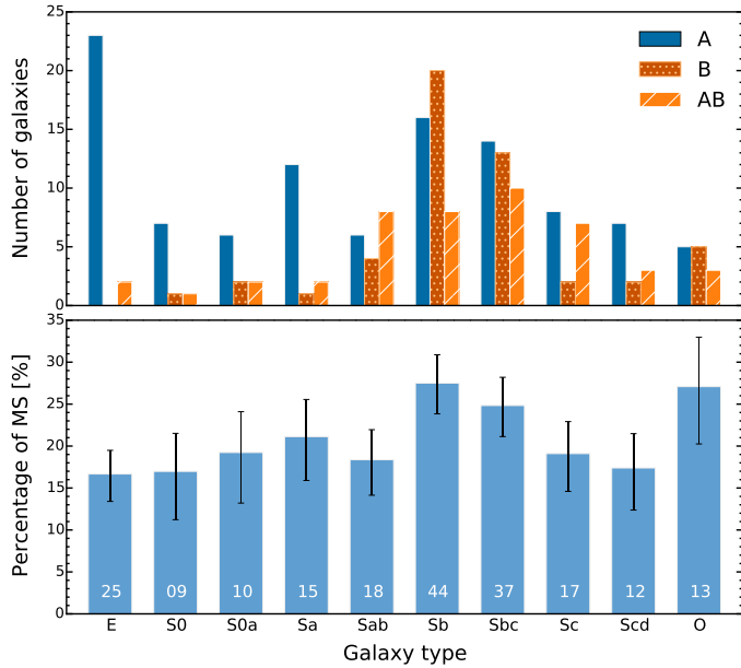
Fig. 5. Distribution of visually classified morphological types in the DR2 sample. We divide the galaxies into ellipticals (E), spirals (from S0 to Scd), and the other group “O”, which includes Sd, Sdm, Sm, and I (only one) types. Upper panel: bar strength histogram, where A stands for non-barred, B for barred and AB if unsure. Lower panel: the percentage of galaxies in the DR2 sample with respect to the CALIFA MS distribution. The total number of galaxies in the DR2 for each morphology type is written on each bar. Error bars are computed from the binomial errors of the associated DR2 number counts (Wilson 1927). The morphological distribution of the DR2 sample is similar to that of the mother sample.
