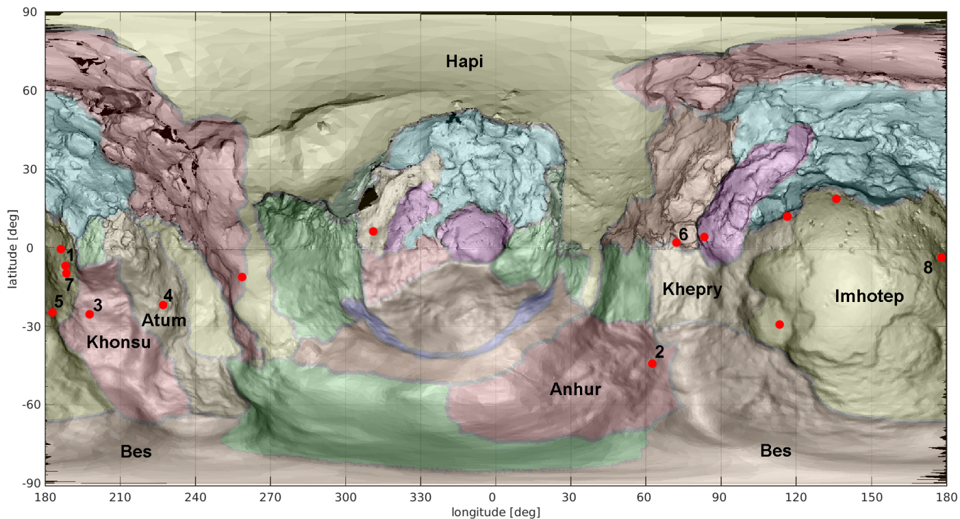
Fig. 1. Map of comet 67P/Churyumov-Gerasimenko resulting from merging a more detailed shape model SHAP4S (Preusker et al. 2015) for the northern hemisphere and shape model SHAP5 (Jorda et al. 2016) for the southern hemisphere. In red are reported the selected bright spots, based on OSIRIS images and a spectro-photometric analysis, considered as good targets to be investigated by an analysis of VIRTIS data, plus the two bright spots analysed by Filacchione et al. (2016a). The numbers (1-8) represent the spots with positive detection of H 2 O ice by VIRTIS analysis discussed in this paper.
