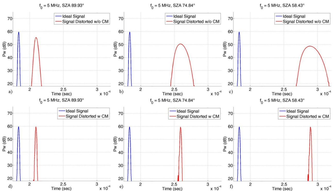
534 535 Fig. 14. Comparison between the ideal and the distorted signal for orbit 4646. Both signal are range compressed. The 536 effects of the distortion, as the delay and a wide main lobe, are clearly visible.
