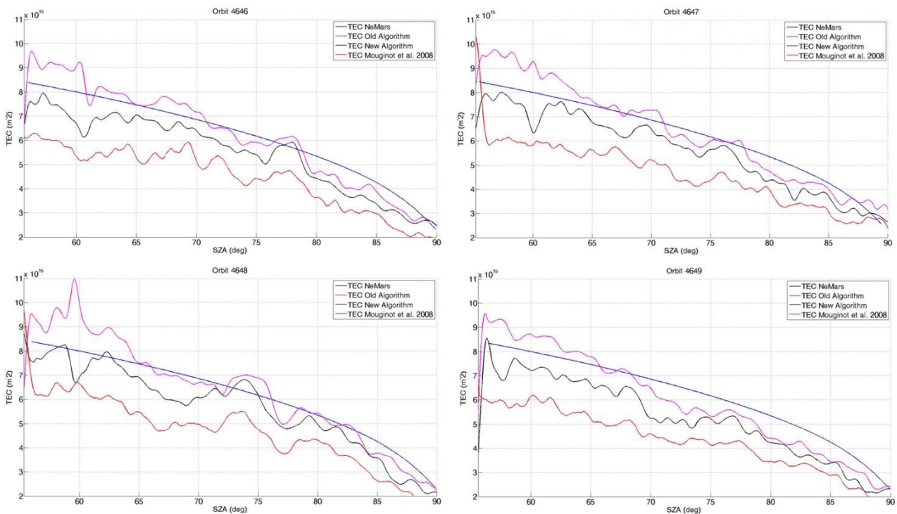
514 515 Fig. 13. TEC comparison for orbits 4646-4647-4648-4649. The blue line shows the NeMars TEC, the magenta line 516 shows the old TEC, the black line shows the TEC estimated with the new algorithm while the red line shows the one 517 from Mougnot et al. (2008).
