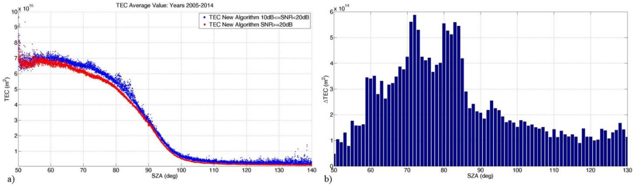
391 a) Fig. 9 TEC from the new algorithm averaged over 0.01° SZA bins, plotted as a function of SZA, considering signals 392 with a SNR≥20dB (red points) and the ones evaluated for 10dB≤SNR<20dB (blue points) (a). Averaged difference, 393 over 1° SZA bins as a function of SZA (b). 394
