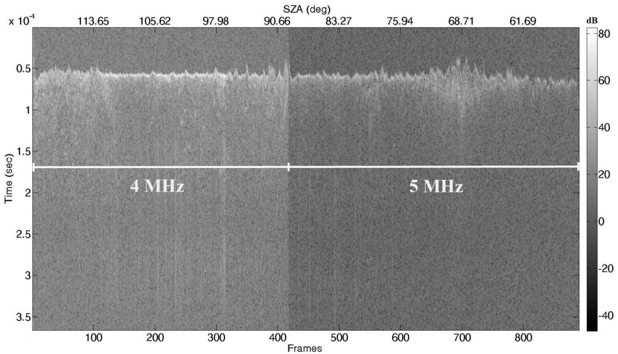
192 Fig. 1. Orbit 4646 radargram. The signal is range compressed with the CM, but the tracking trigger is not removed, so 193 the surface and subsurface topography information are lost. The different brightness is related to the different gain used 194 by the Automatic Gain Control (AGC) for each frequency.
