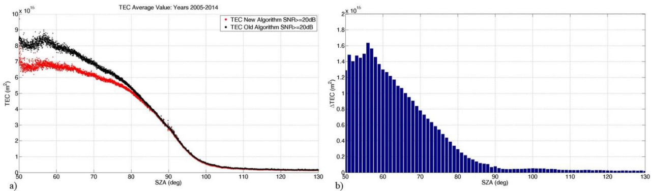
372 373 Fig. 8. TEC, averaged over 0.01° SZA bins, plotted as a function of SZA, considering signals with a SNR \geq 20 dB (a). 374 Averaged difference, between new TEC and old TEC, over 1° SZA bins as a function of SZA, considering signals with 375 a SNR \geq 20 dB (b)
