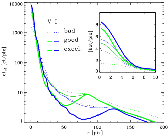
Fig. 13. Normalized radial profiles \text{ct}_{\text{th6}} for V- and N_I-band observations of HD 161096 with “excellent”, for HD 183143 with “good”, and HD 129502 with “bad” quality PSFs.
