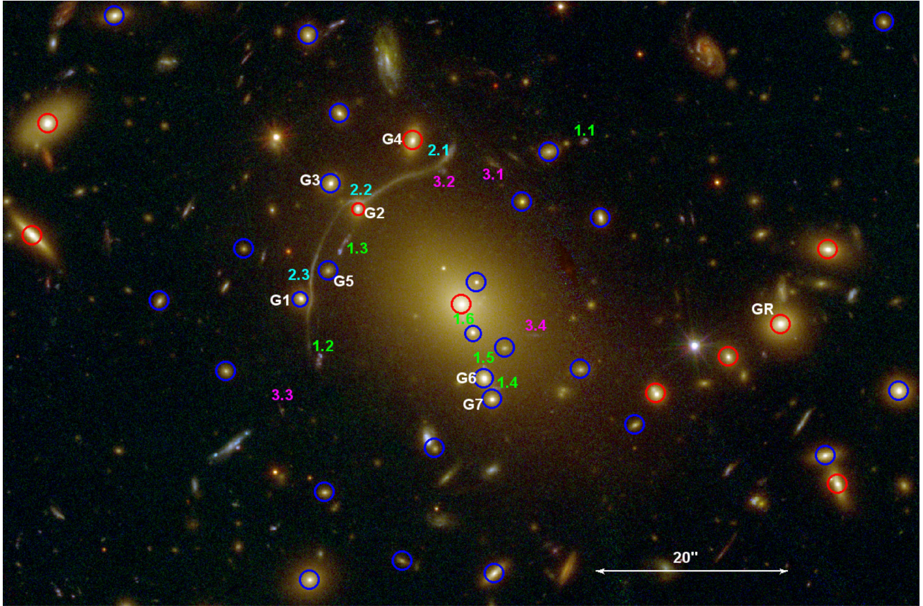
Figure 1. Colour composite image of the core ( \sim 1.5 arcmin \times 1.5 arcmin) of A611 created using the CLASH HST data set: blue = F435W + F475W ; green = F606W + F775W + F814W + F850LP ; red = F105W + F110W + F140W + F160W . Blue circles mark the cluster members included in the SL analysis. Red circles mark the galaxies with measured central velocity dispersions. ‘GR’ indicates the galaxy used as reference for the luminosity scaling relation. ‘G1’ to ‘G7’ are the galaxies we model individually. The three multiply-lensed systems used in the SL analysis are labelled in green (system 1), cyan (system 2) and magenta (system 3). North is up and east is left.
