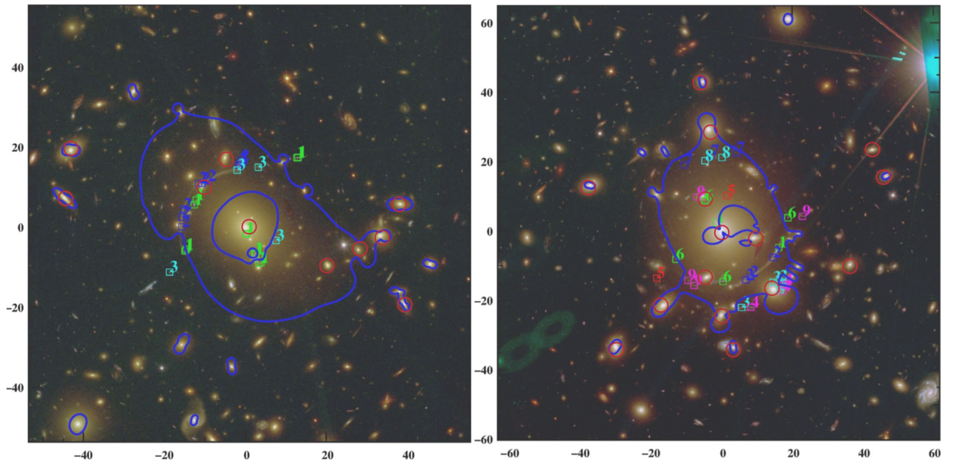
Figure 5. HST colour composite images of A611 ( z = 0.288 ; left) and A383 ( z = 0.189 ; right). We show the multiple image (numbered), the cluster members with measured \sigma_{\text{sp}} (red circles), and the critical lines for a source at redshift z_s = 2 (blue). Axis labels are in arcseconds with respect to the BCG.
