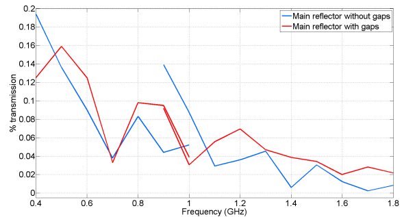
Fig. 4. Percentage transmission for SKA Band 1 and 2 of the main reflector with gaps compared to a solid reflector without gaps.
