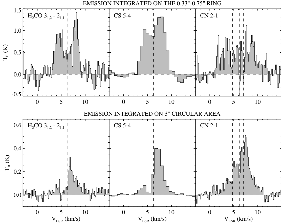
Fig. B.1. \text{H}_2\text{CO } 3_{1,2}-2_{1,1} , \text{CS } 5-4 , and \text{CN } 2-1 spectra integrated over a 0'.33-0'.75 ring area ( top panels ) and over a 3'' circular area ( bottom panels ), in brightness temperature T_B . The vertical dashed lines indicate the systemic velocity, V_{\text{sys}} = +6.24 \text{ km s}^{-1} . For \text{CN } 2-1 the velocity scale corresponds to the brightest of the three hyperfine components at 226.87 \text{ GHz} reported in Table 1 ( N=2-1 , J=5/2-3/2 , F=7/2-3/2 ), and the position of the two fainter components is indicated by the vertical dashed lines.
