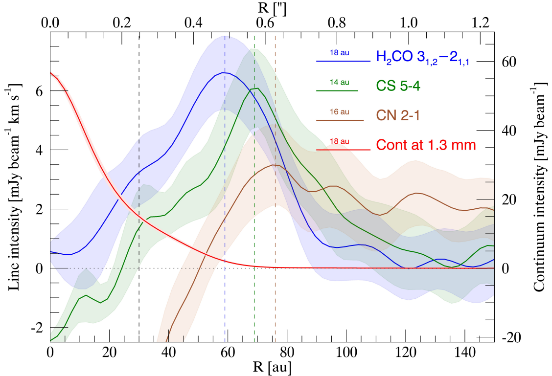
Fig. 2. Azimuthally averaged radial intensity profile of \text{H}_2\text{CO } 3_{1,2}-2_{1,1} (blue), \text{CS } 5-4 (green), and \text{CN } 2-1 (brown; blending of the three components at 226.87 GHz reported in Table 1) in \text{mJy beam}^{-1} \text{ km s}^{-1} (left axis), and of the 1.3 mm continuum (red) in \text{mJy beam}^{-1} (right axis). The radial distance is indicated in au on the bottom axis and arcseconds on the top axis. The angular resolution of the lines/continuum profiles is indicated by the corresponding horizontal lines. The shaded areas indicate the dispersion of the intensity values around the mean along each annulus in the radial direction. The vertical dashed lines indicate the position of the CO snowline (black), and of the peaks of the emission in \text{H}_2\text{CO } 3_{1,2}-2_{1,1} (blue), \text{CS } 5-4 (green), and \text{CN } 2-1 (brown).
