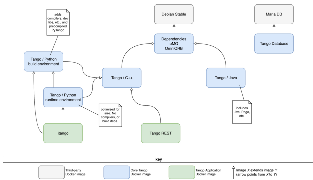
Figure 3: SKA-docker project module view.
