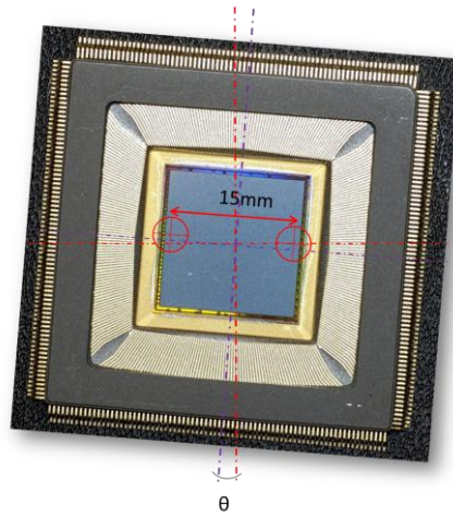
Figure 3 Representation of the possible ASIC alignment error ( \theta ) which translate in a systematic error on the polarization angle knowledge.
