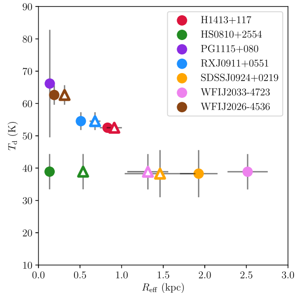
Figure 7. The effective radius ( R_{\text{eff}} ) of the dust continuum (solid circles) and CO line emission (open triangles) against effective dust temperature ( T_d ) for the seven lensed quasar hosts investigated here.
