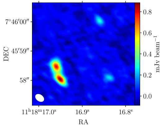
Figure 3. ALMA 346 GHz continuum images of PG 1115+080 with natural weighting of the visibility data. The synthesized beam FWHM is shown in the bottom left-hand corner.
