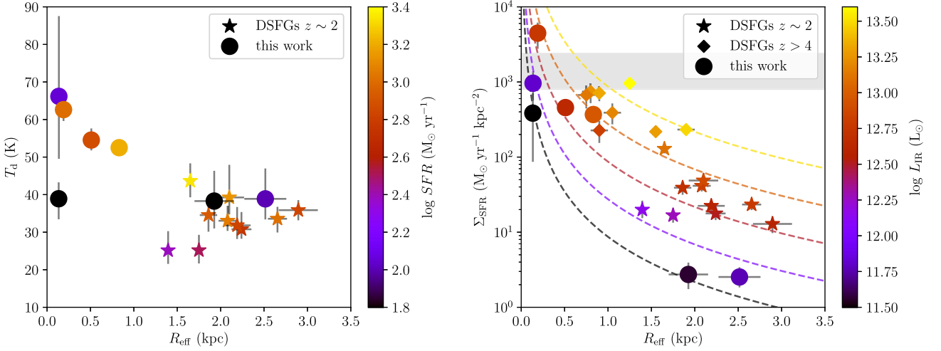
Figure 8. Left: Effective radius ( R_{\text{eff}} ) against effective dust temperature ( T_d ), coloured by SFR. Right: Effective radius against mean SFR surface density ( \Sigma_{\text{SFR}} ), where the grey region shows our estimated Eddington limit and its uncertainty. \Sigma_{\text{SFR}} and the dashed curves show the tracks for \log L_{\text{IR}} values of 11.5, 12, 12.5, 13, and 13.5. Circles show the quasar hosts in this work (with H1413+117 corrected for SED blending); stars show coeval DSFGs at z \sim 2 (Hodge et al. 2016, 2019); triangles show DSFGs at z > 4 (Riechers et al. 2013, 2014, 2017; Hodge et al. 2015, 2016). Four of the seven quasar hosts have SFR surface densities close to the Eddington limit, similar to DSFGs selected at z > 4 .
