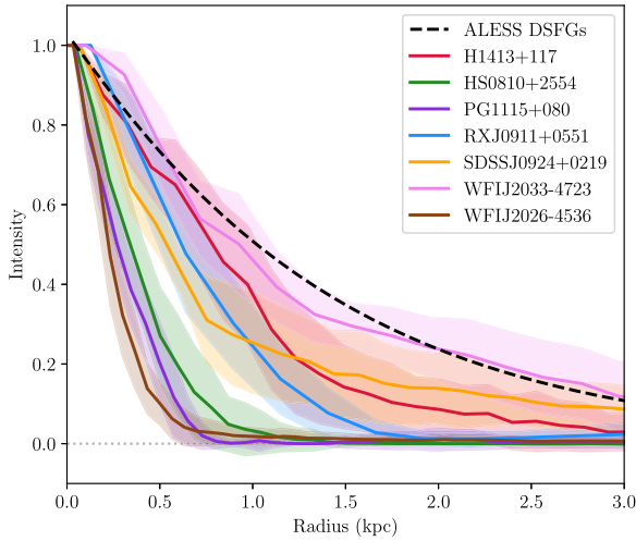
Figure 6. Normalized, azimuthally averaged surface brightness profiles of the reconstructed dust emission from the quasar hosts, accounting for ellipticity. The shaded regions show the respective standard deviation of the dust emission. The radius of HS 0810+2554 and PG 1115+080 is scaled to the size of the minor axis, based on the axial ratio from the Sérsic model fits (see Section 4.1). The black dotted line shows the mean profile of (unlensed) ALESS DSFGs from Sérsic fits (Hodge et al. 2016, 2019).
