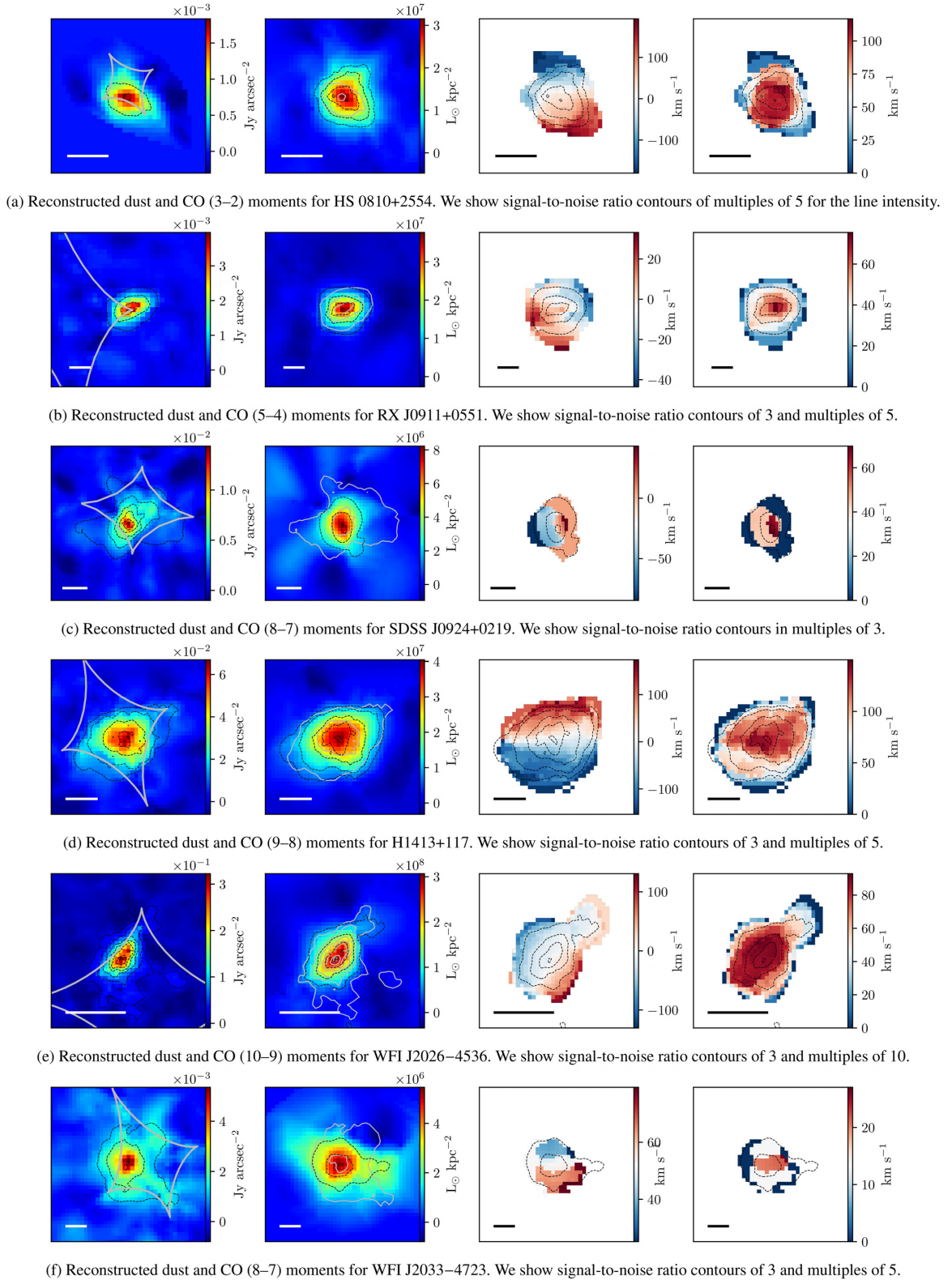
Figure 4. Reconstructed dust emission and moment maps for the six lensed quasar systems with spectral line data. The dust emission is shown in units of \text{Jy arcsec}^{-2} with the lensing caustics shown in grey. Dashed contours show signal-to-noise ratio contours, starting at 3. Continuum contours are shown in grey over the moment 0 image. The bar shows 1 kpc at the redshift of the source. The line reconstructions are generated by masking pixels in each channel below 3\sigma . The CO velocity is corrected to the redshift derived from a Gaussian fit to the CO line profile.
