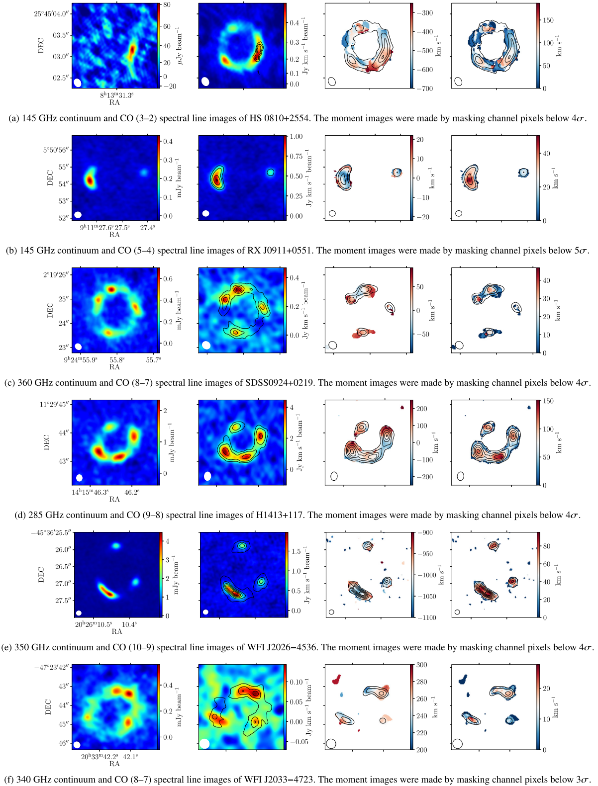
Figure 2. Deconvolved ALMA images for the six systems with spectral line data, using natural weighting of the visibilities. Left to right: the continuum; moment 0 (velocity-integrated line intensity); moment 1 (line velocity); moment 2 (velocity dispersion). The beam FWHM is shown in the lower left corner.
